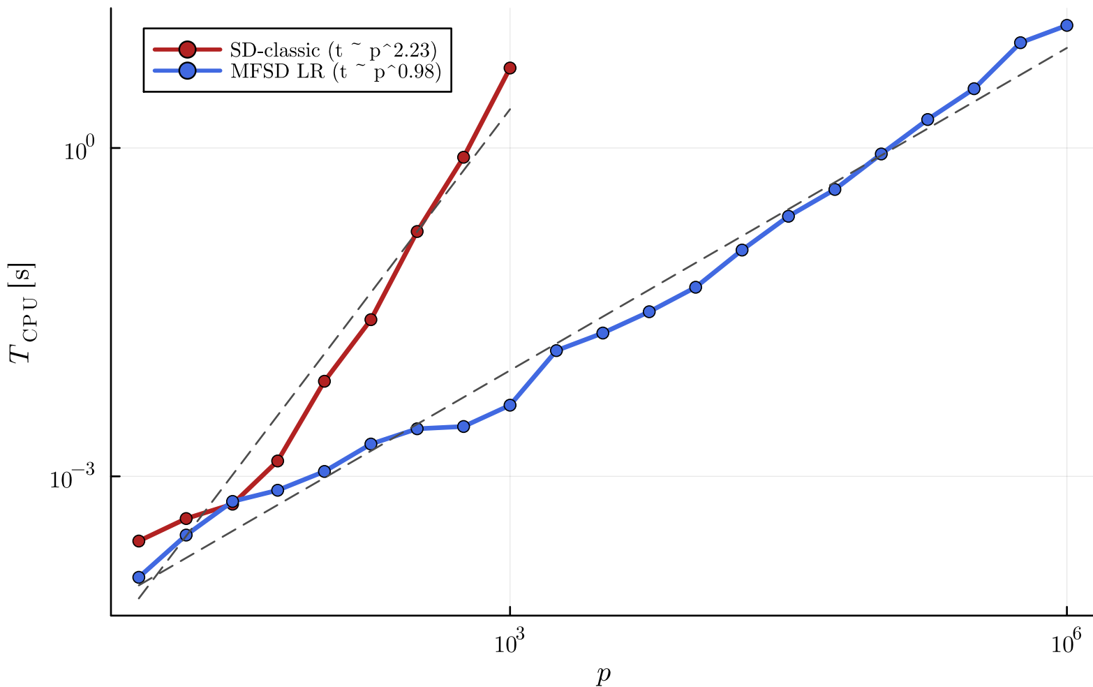
SD-classic vs multiplication-free LR mapping
