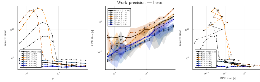
Figure 9. Work-precision — FEM beam with delayed boundary feedback.
