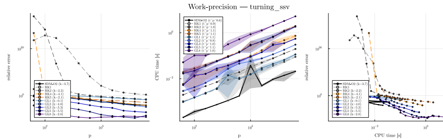
Figure 8. Work-precision — turning with spindle-speed variation.
