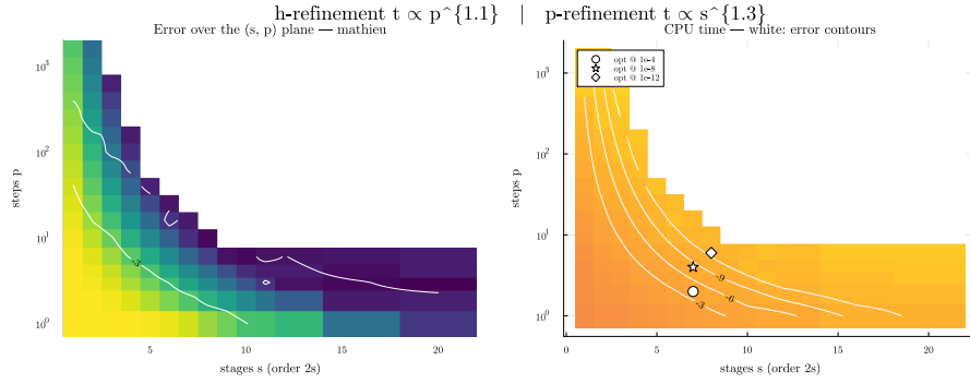
Figure 6. The (s, p) -map for the low-demand delayed Mathieu equation (compare Figure 5): here deep accuracy is reached in the high-order/low- p region as well, and the optima sit near the spectral corner because the matrices stay tiny.
