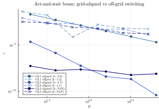
Figure 12. Act-and-wait beam: relative error versus p for GL1–GL3 on grid-aligned (solid) and off-grid (dashed) meshes.
