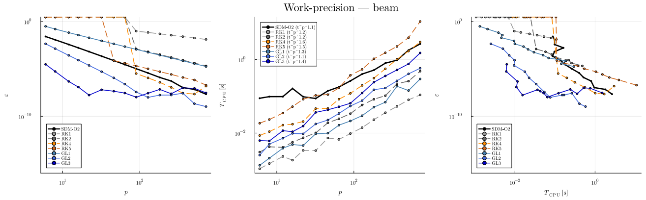
Figure 11. Work–precision study for the FEM beam with delayed boundary feedback. The error axis is clipped at 3 \cdot 10^0 : below the CFL-like stability bound the explicit methods produce meaningless values (up to 10^{43} ), which carry no information beyond “unstable”. CPU times are minima of repeated warm-started benchmark measurements.
