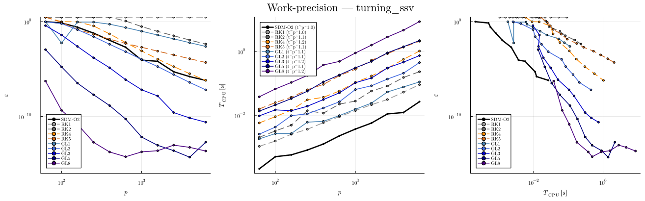
Figure 10. Work–precision study for the turning system with spindle-speed variation; same panel logic as Figure 3, parameters in Appendix A.
