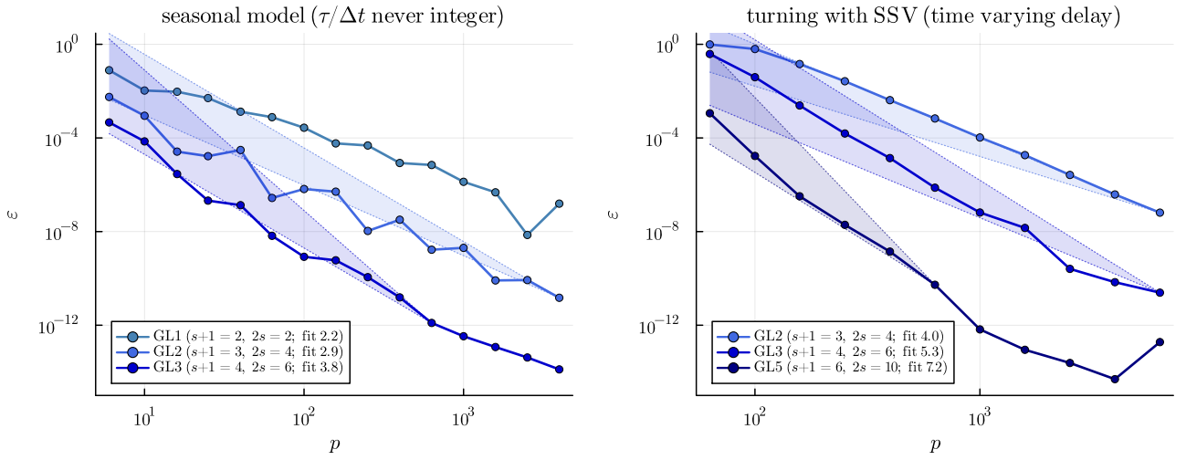
Figure 7. Convergence of the dominant multiplier for non-mesh-commensurate delays: seasonal model (left) and SSV turning system (right). Shaded bands span the order bracket [s+1, 2s] per method (dotted edges), anchored at the finest pre-floor point; legend entries give the fitted log-log slope. All curves remain inside their bands: the seasonal model presses the interpolation-limited s+1 edge, whereas the SSV system retains orders up to the superconvergent cap. The GL5 plateau at \varepsilon \approx 10^{-13} marks the accuracy of the two-resolution reference, not of the method.
