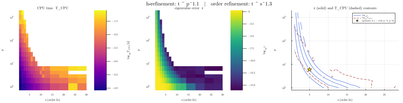
Figure 8. The (s, p) -map for the low-demand delayed Mathieu equation (same three panels as Figure 5): here deep accuracy is reached in the high-order/low- p region as well, and the optima sit near the spectral corner because the matrices stay tiny; the polynomial CPU growth along s is nevertheless visible at the extended stage orders.
