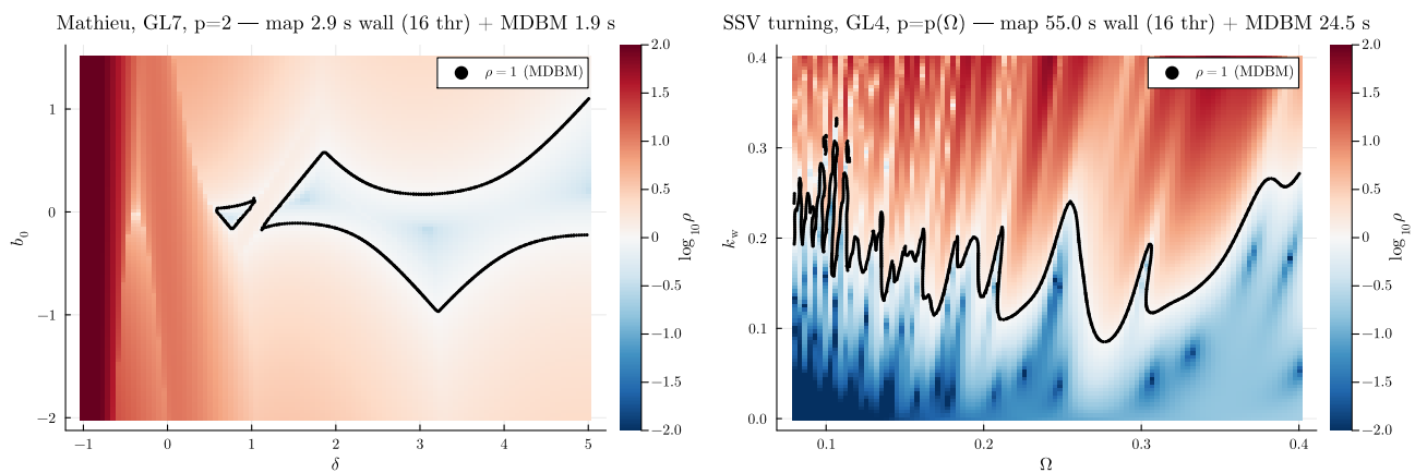
Figure 13. Brute-force stability charts at the optimal settings, coloured by \log_{10} \rho (blue: stable, red: unstable); black dots: the \rho = 1 boundary refined by MDBM; the measured CPU times appear in each title. Left: delayed Mathieu equation in the (\delta, b_0) plane ( \epsilon_M = 1 , a_1 = 0.1 , \tau = T = 2\pi ), GL7 with p = 2 . Right: SSV turning in the (\Omega, k_w) plane with strong modulation ( \zeta = 0.02 , A_{SSV} = 0.3 , N_T = 10 ); here the step count follows the sampling recipe of Section 6 per point, p(\Omega) = \lceil 16/\Omega \rceil — the paper's own rule applied in a realistic production setting. Grid evaluation on 16 threads; the MDBM refinement is serial.
