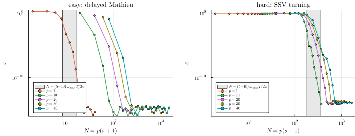
Figure 6. Order refinement at the fixed step counts p = 1, 10, 20, 30, 40 : relative error versus the total sample count N = p(s+1) for the easy (left) and hard (right) system, error clipped at 3 \cdot 10^0 . The shaded band is the sampling estimate (10) with c_s = 5-10 . Superconvergent decay starts only once N crosses the band, whose position is set by the oscillation content \omega_{\max} T / 2\pi of the system — not by the method order; on the hard system the single-step curve ( p = 1 ) cannot reach the band within the practical stage range and stays meaningless throughout.
