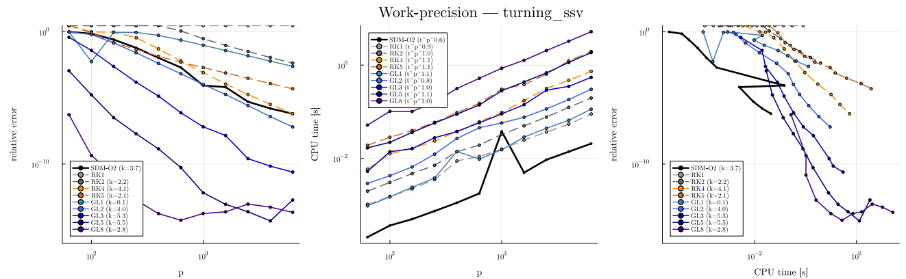
Figure 9. Work-precision — turning with spindle-speed variation.
