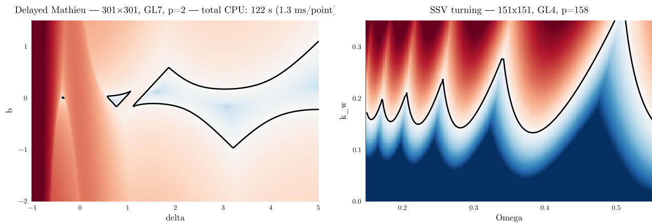
Figure 12. Brute-force stability charts at the optimal settings, coloured by \log_{10} \rho (blue: stable, red: unstable), black curve: stability boundary \rho = 1 ; the measured total CPU time appears in each title. Left: delayed Mathieu equation in the (\delta, b) plane ( \varepsilon = 1 , a_1 = 0.1 , \tau = T = 2\pi ), GL7 with p = 2 . Right: SSV turning in the (\Omega, k_w) plane with strong modulation ( \zeta = 0.02 , A_{SSV} = 0.3 , N_T = 10 ); here the step count follows the sampling recipe of Section per point, p(\Omega) = \lceil 16/\Omega \rceil — the paper's own rule applied in production. All computations single-threaded.
