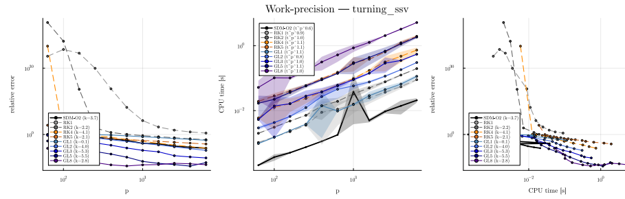
Figure 6. Work-precision — turning with spindle-speed variation.
