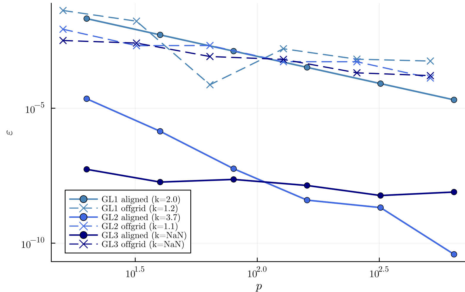
Act-and-wait beam: grid-aligned vs off-grid switching
