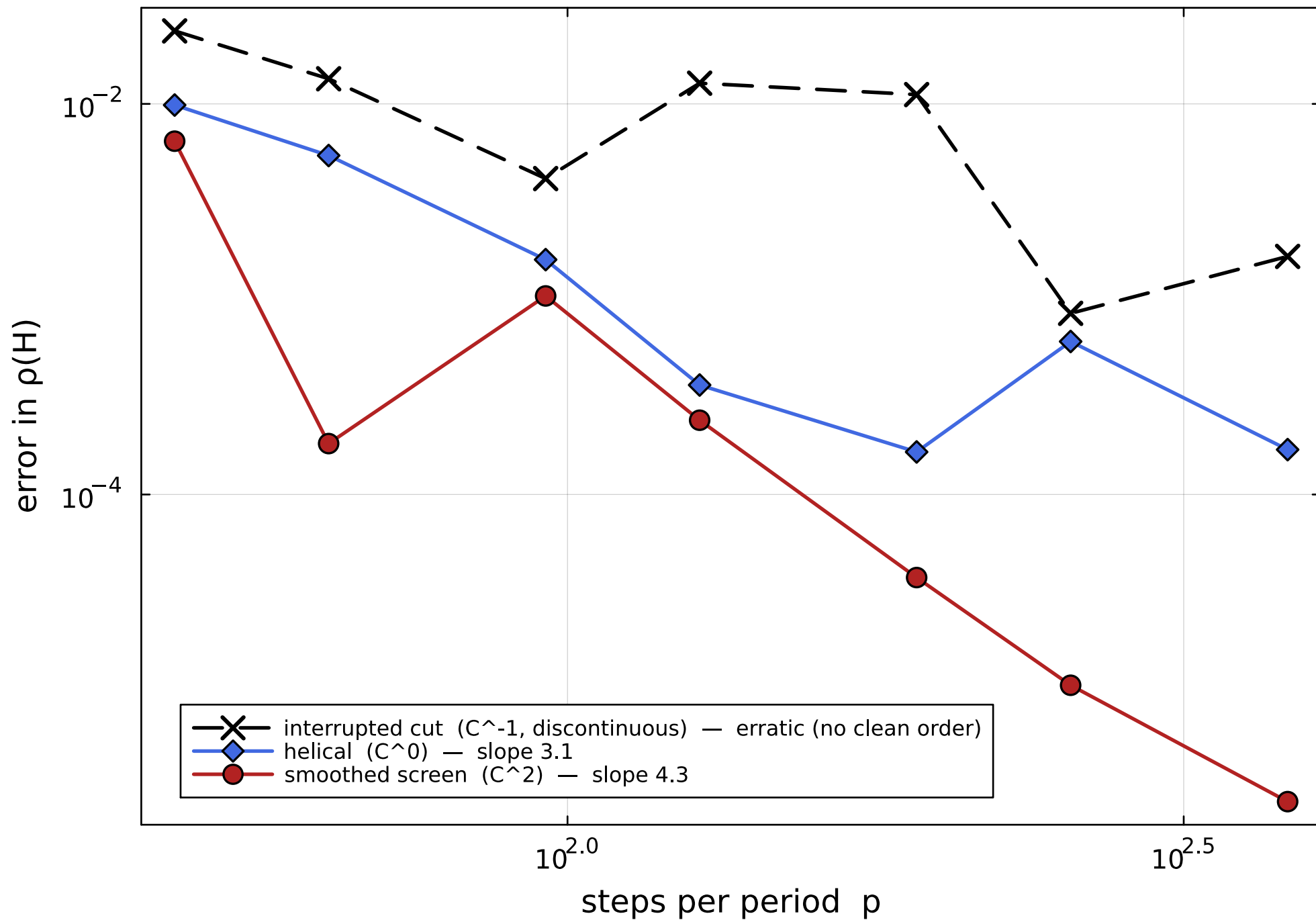
SSV milling: collocation order vs engagement regularity (S=3)
