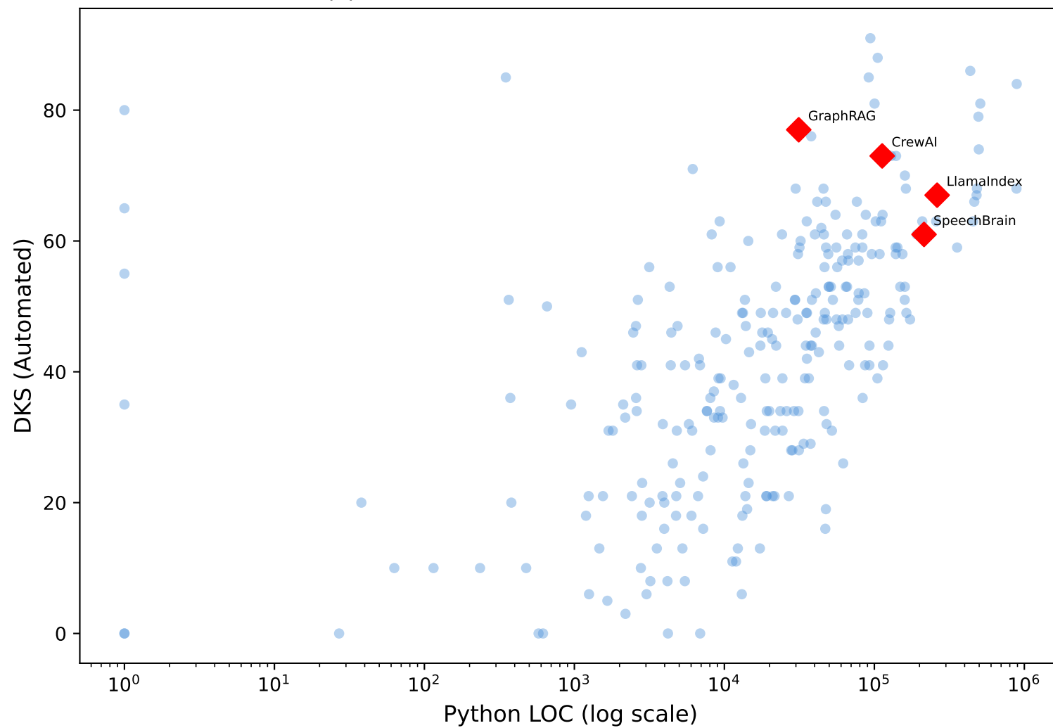
(c) DKS vs Code Size — Externals in Red
