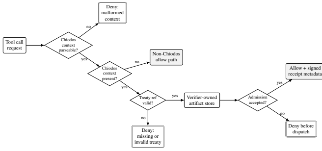
Figure 1: Pre-dispatch admission. A federated request without valid treaty context is denied before tool invocation.
