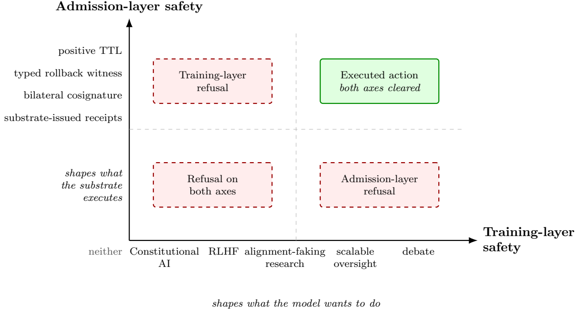
Figure 2: Composition of training-layer and admission-layer safety as orthogonal axes. A tool call is executed only when both axes clear; training-layer interventions (Constitutional AI, RLHF, alignment-faking research, scalable oversight, debate) shape model behavior along one axis, while admission-layer constraints (positive TTL, typed rollback witness, bilateral cosignature, substrate-issued receipts) shape what the substrate is willing to execute along the other. A scheming model that evades training-layer interventions still faces admission-layer refusal at the point of tool-call evaluation; the three rejection quadrants name the failure modes.
