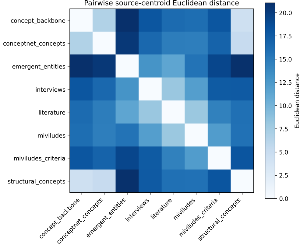
Figure 2: Heatmap of pairwise centroid distances across all eight v2 sources, this run.
