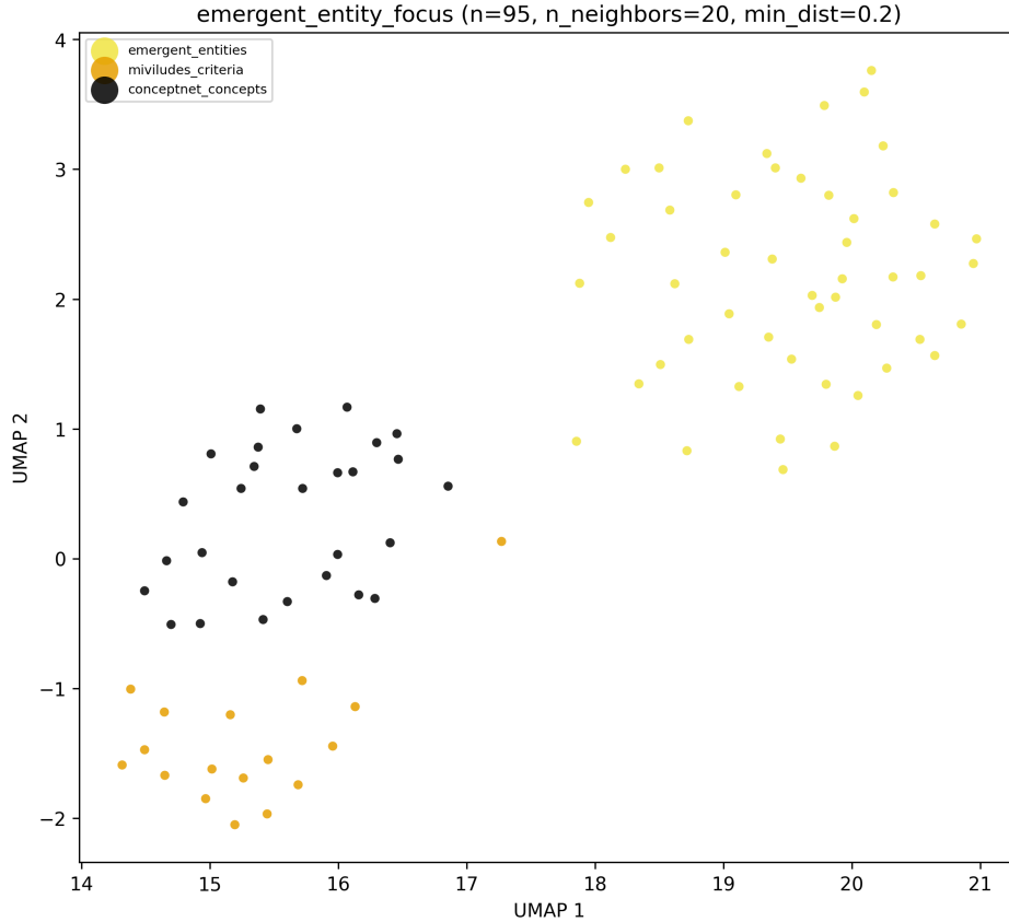
Figure 7: Focused UMAP of the top 50 emergent entities (plus neighbourhood context), coloured by source dataset – the first version of this figure worth showing, now that the entity layer has real content.
