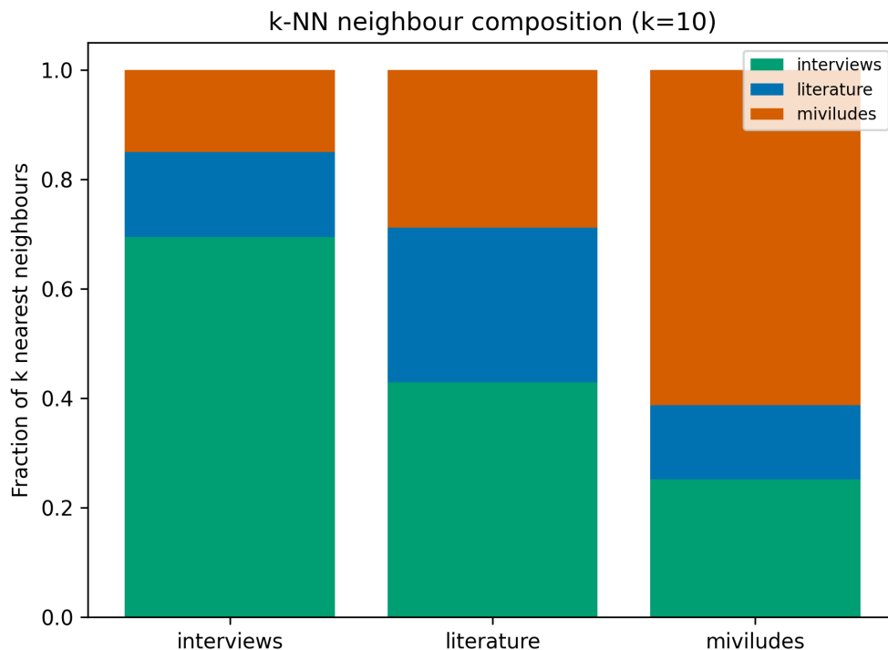
Figure 3: k-NN neighbour composition at k = 10 , equal- n sampling, this run.
