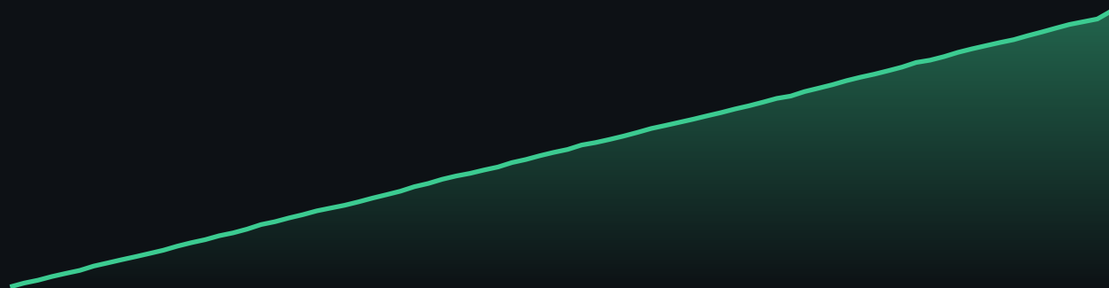
EQUITY CURVE
