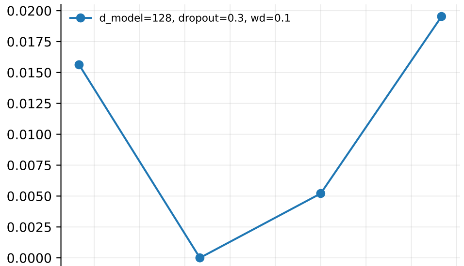
Top-1 accuracy
