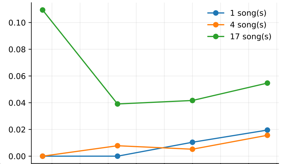
Top-1 accuracy
