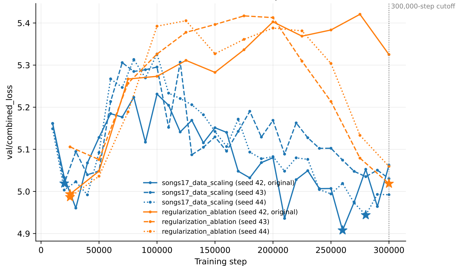
Phase 3 seed-robustness check (steps \leq cutoff)
