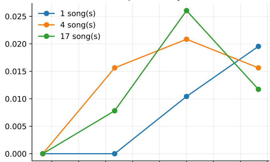
Top-1 accuracy
