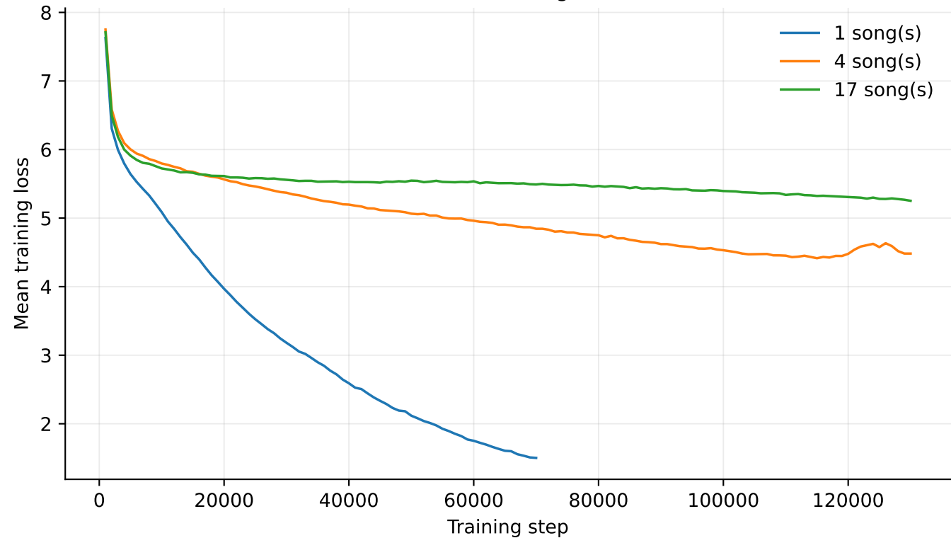
Phase 1 training loss
