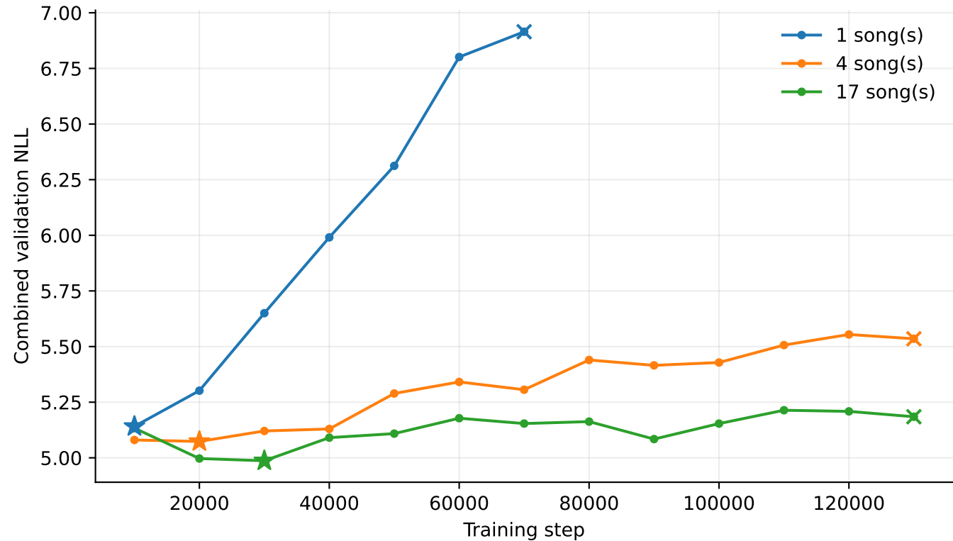
Phase 1 validation loss
