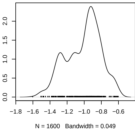
Density of sigma_f
