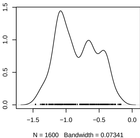
Density of log_prior
