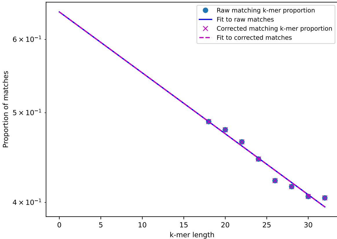
Example fit 2 - SAMN07430859 vs. SAMN10346412
