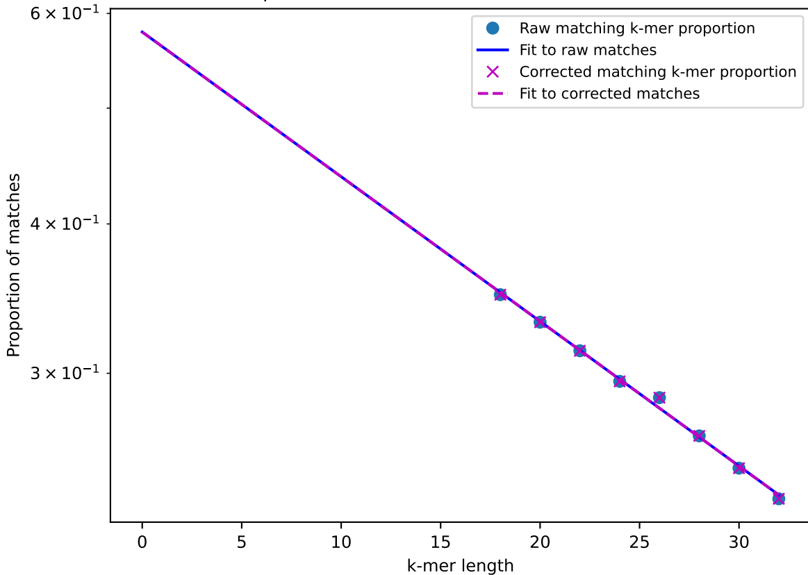
Example fit 3 - SAMEA104452242 vs. SAMN08591168
