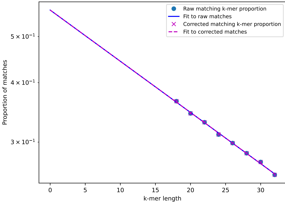
Example fit 5 - SAMN04913894 vs. SAMN10059014
