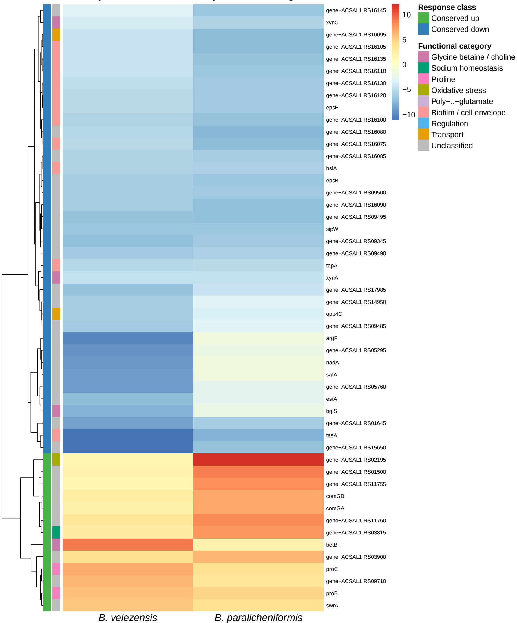
Top 50 conserved salt-responsive orthologs
