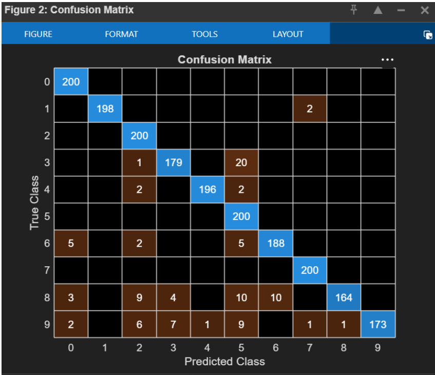
Figure 2: Confusion matrix
