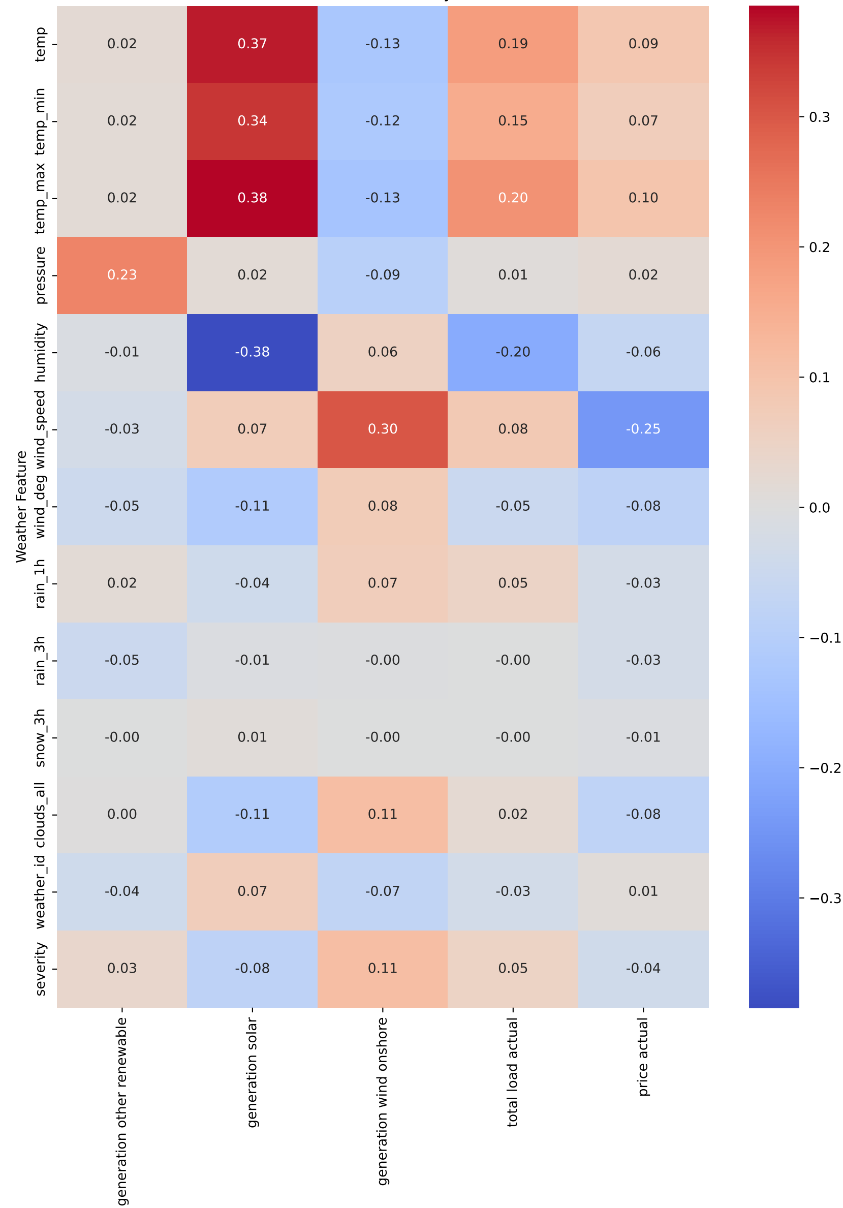
Pearson Correlation: City Madrid
