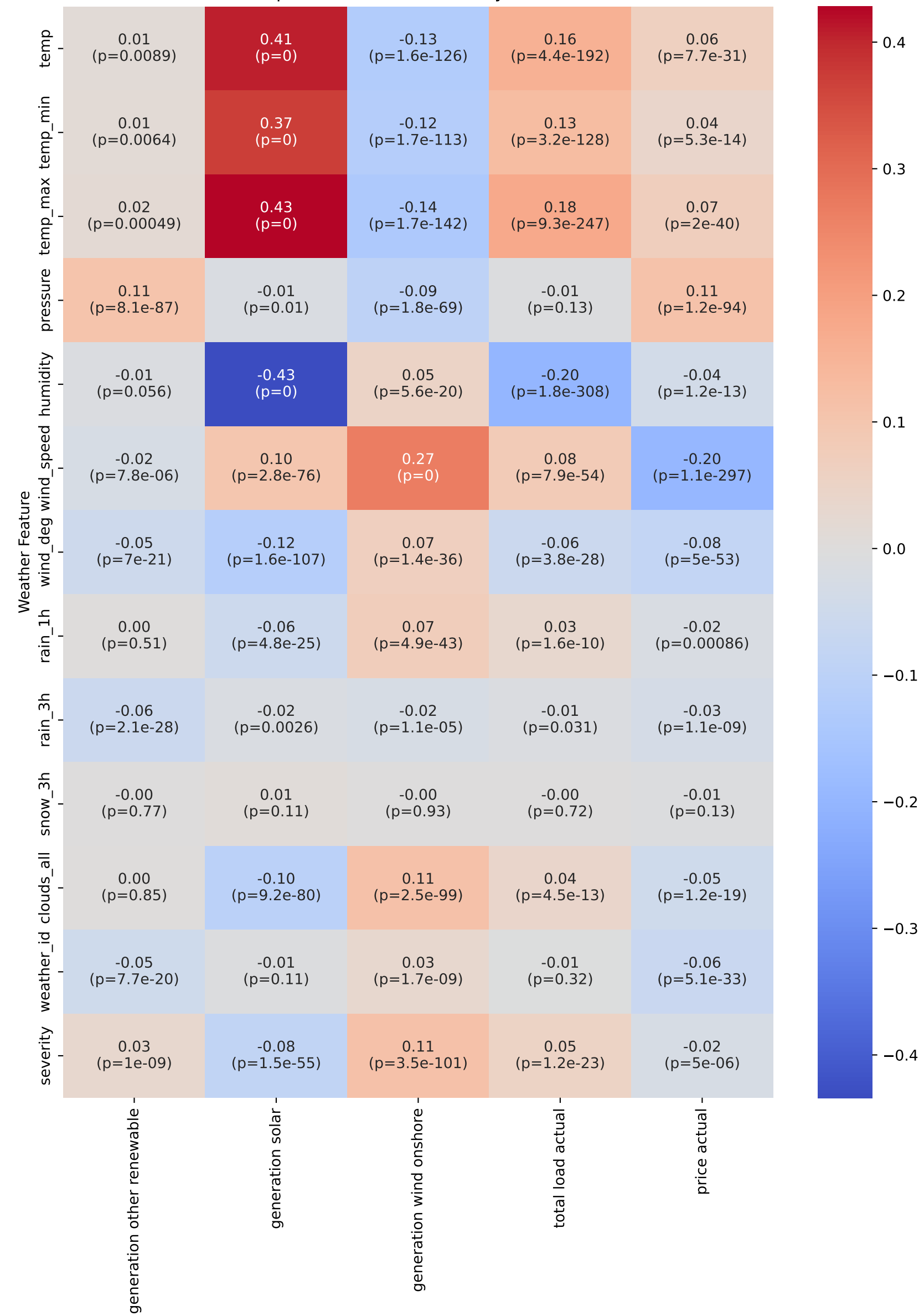
Spearman Correlation: City Madrid
