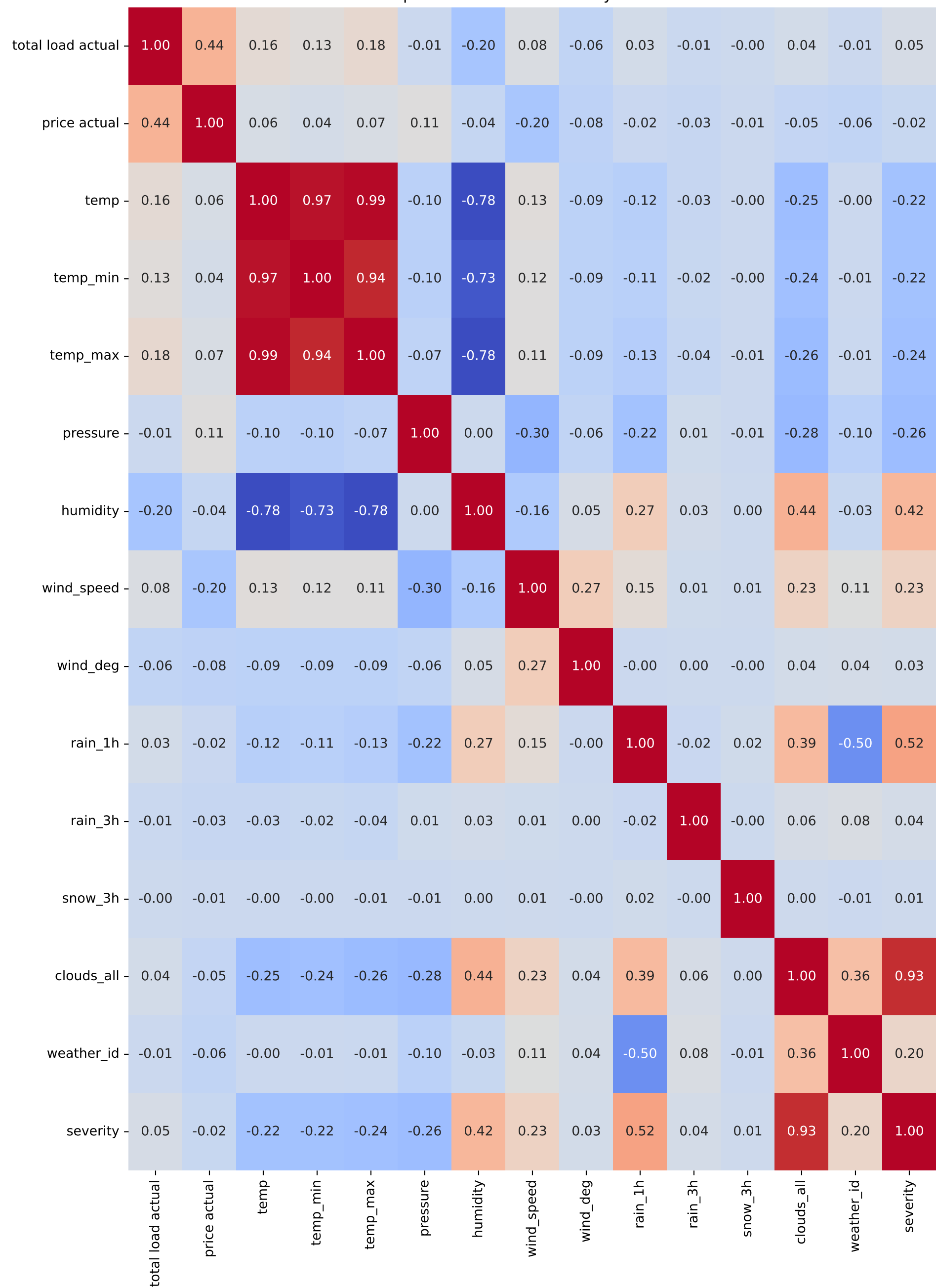
Spearman Correlation - City Madrid
