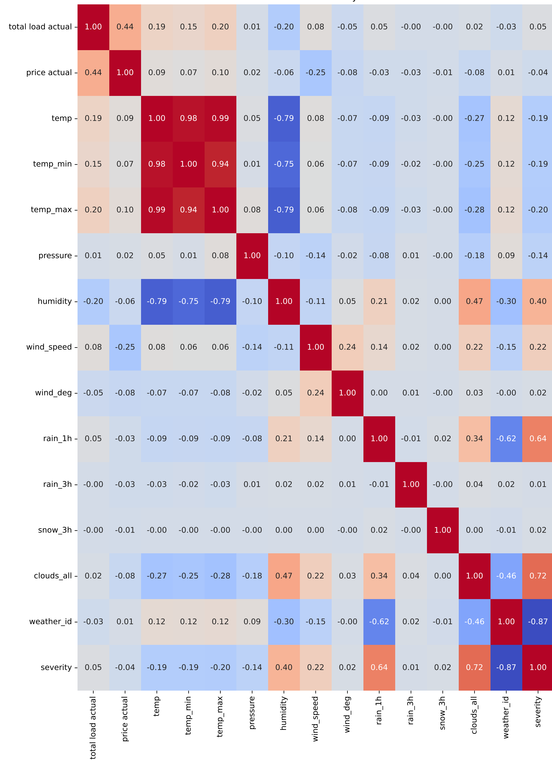
Pearson Correlation - City Madrid
