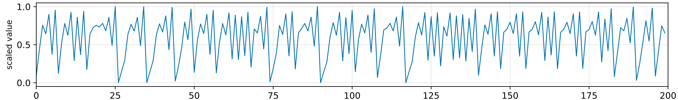
Lorenz-63 — continuous flow, sampled — x-component of the three-dimensional state
