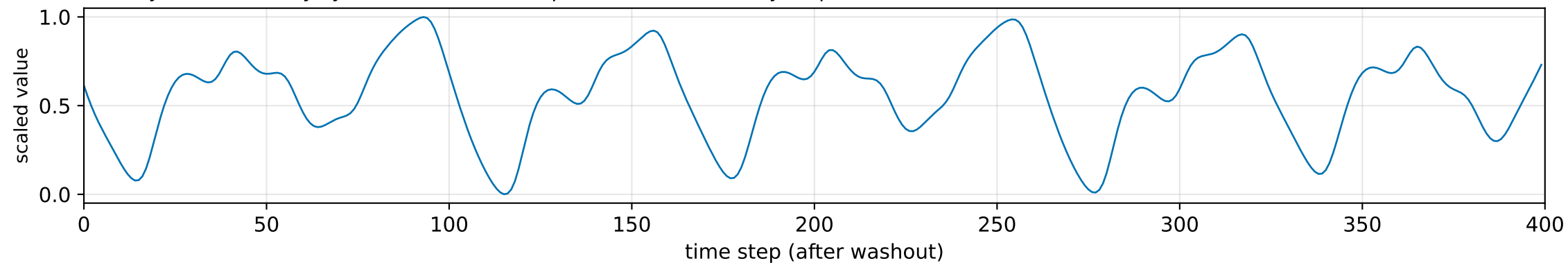
Mackey-Glass — delay system — the state depends on values many steps back
