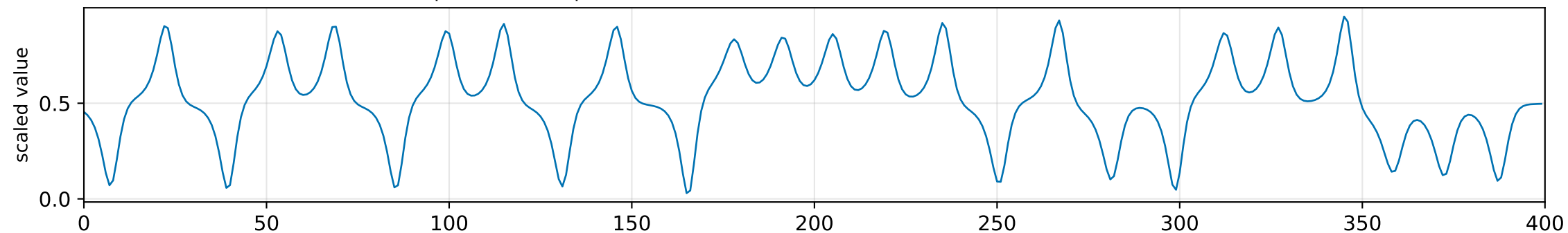
Mackey-Glass — delay system — the state depends on values many steps back
