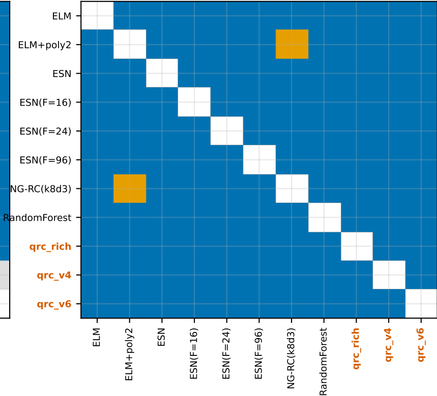
Mackey–Glass
