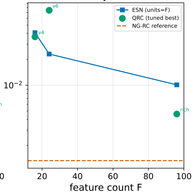
Mackey-Glass
