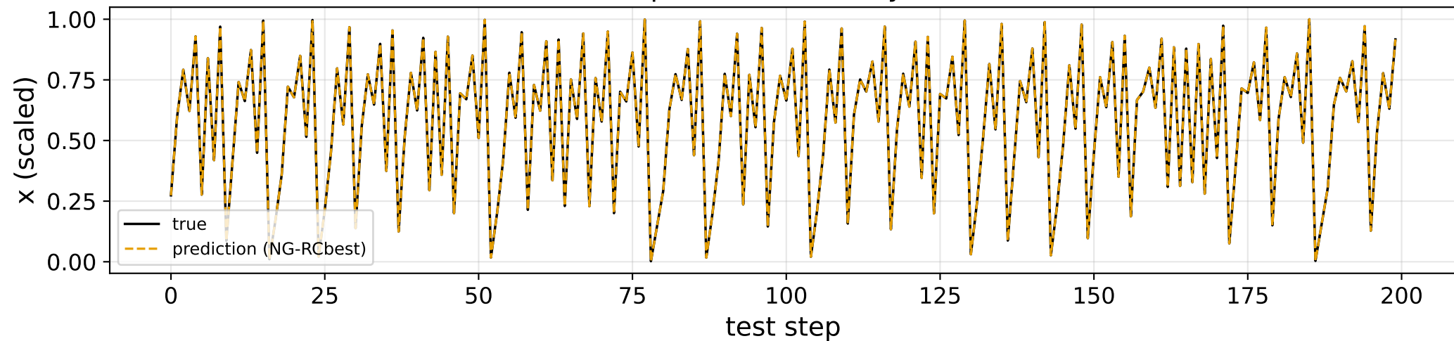
Lorenz-63 — 1-step forecast overlay (test, first 200)
