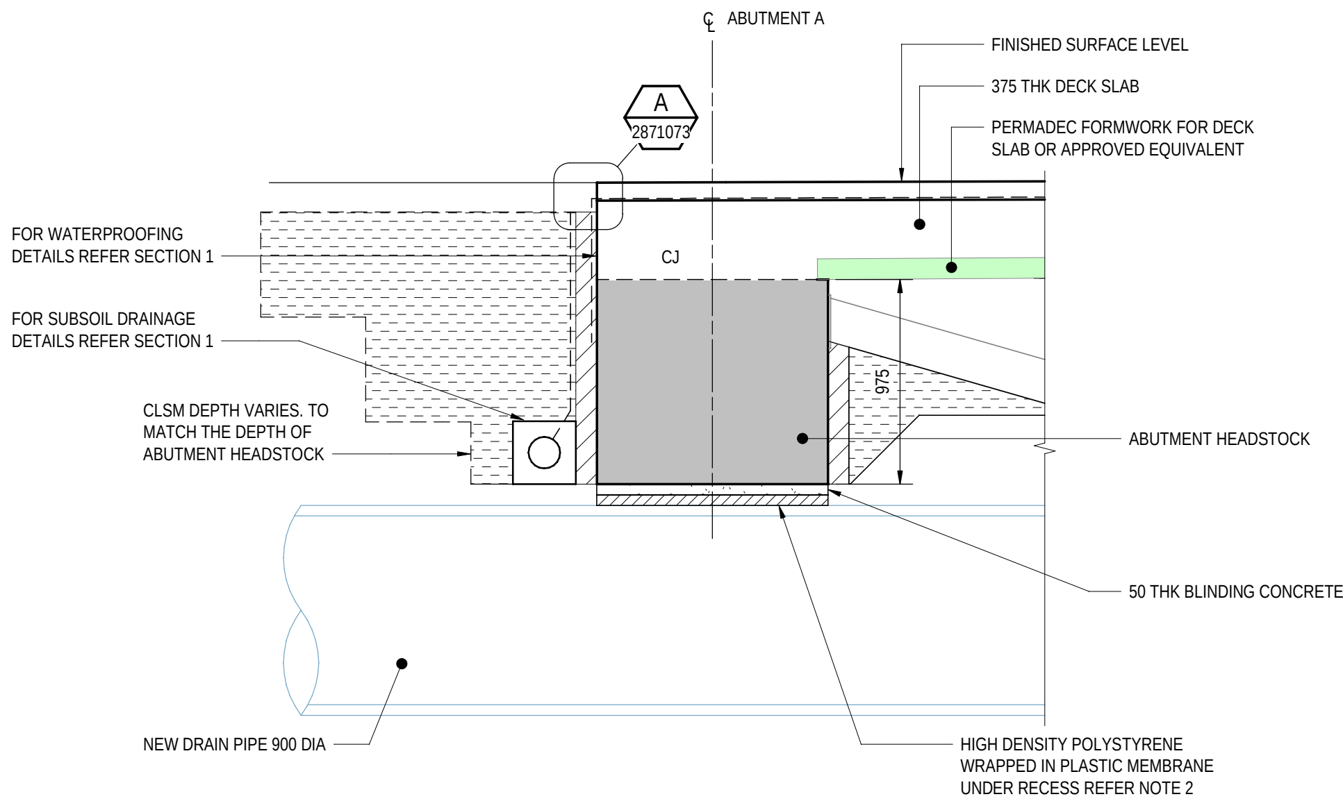
SECTION 3 SCALE 1 : 25 2871071
