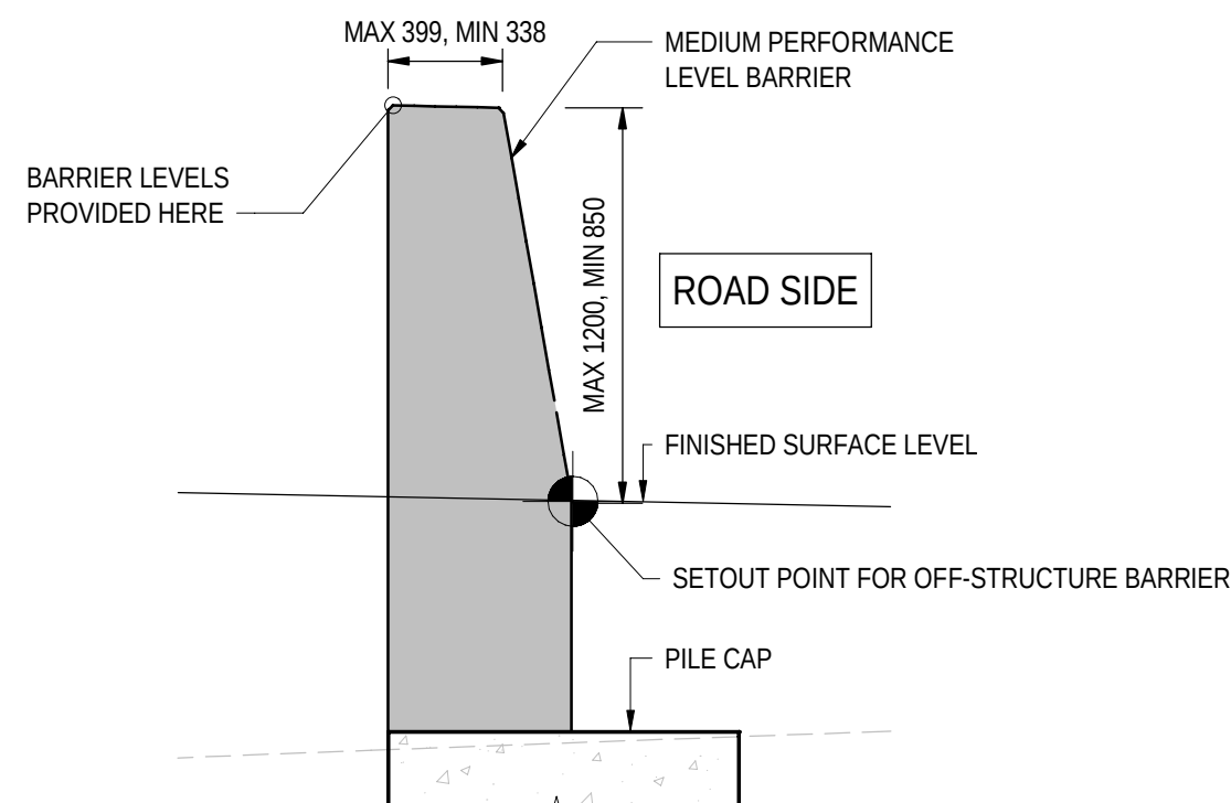
SECTION 5 SCALE 1:25 2871111
