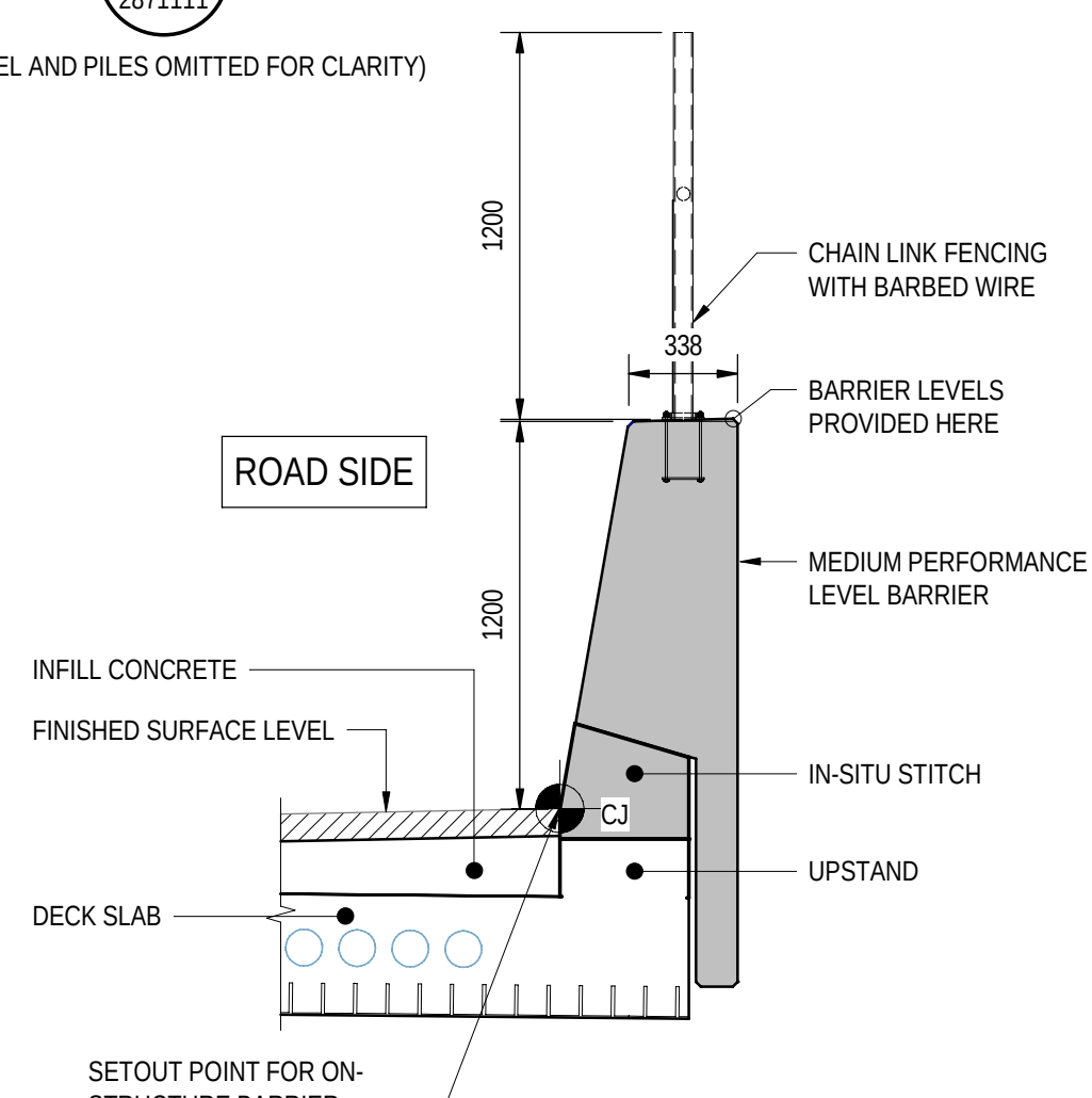
SECTION 4 SCALE 1:25 2871111
