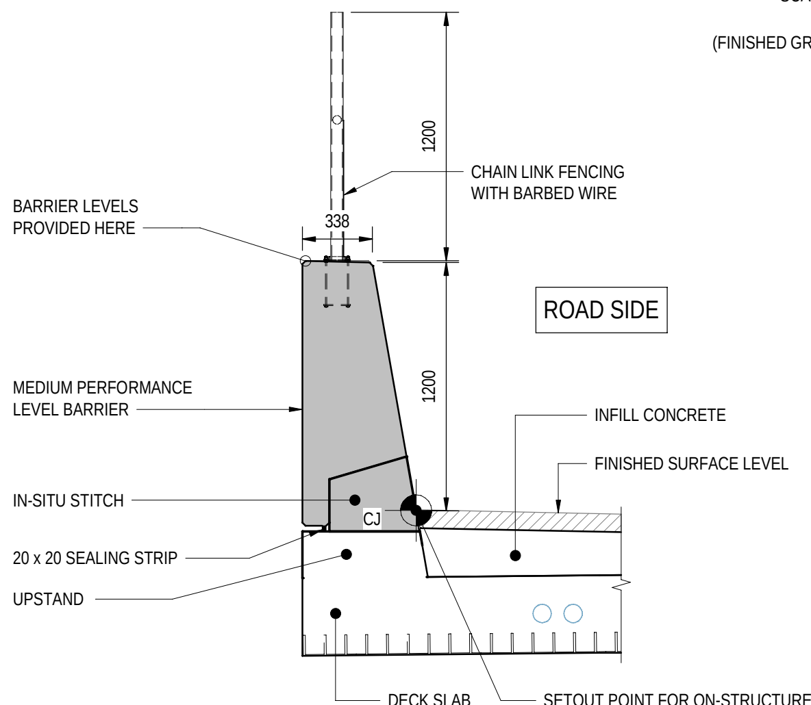
SECTION 3 SCALE 1:25 2871111
