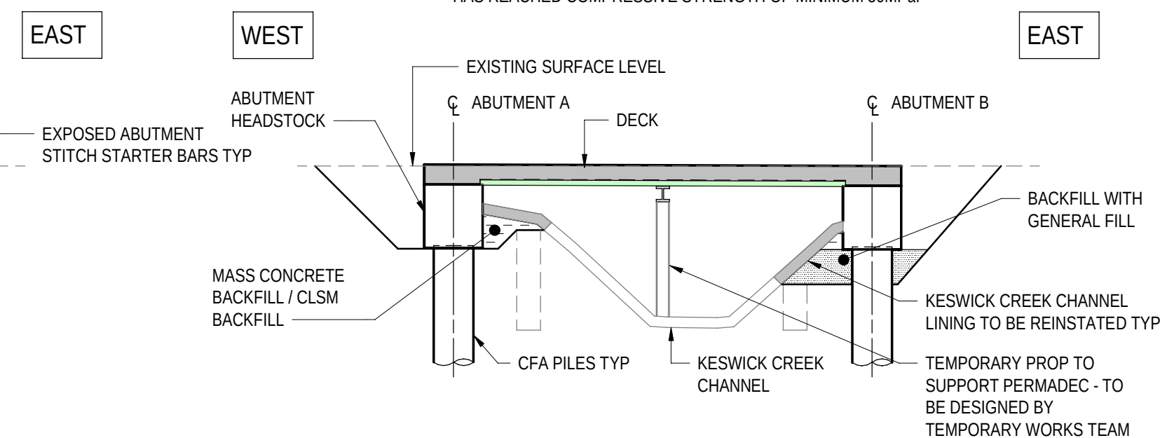
SECTION-STAGE B4
