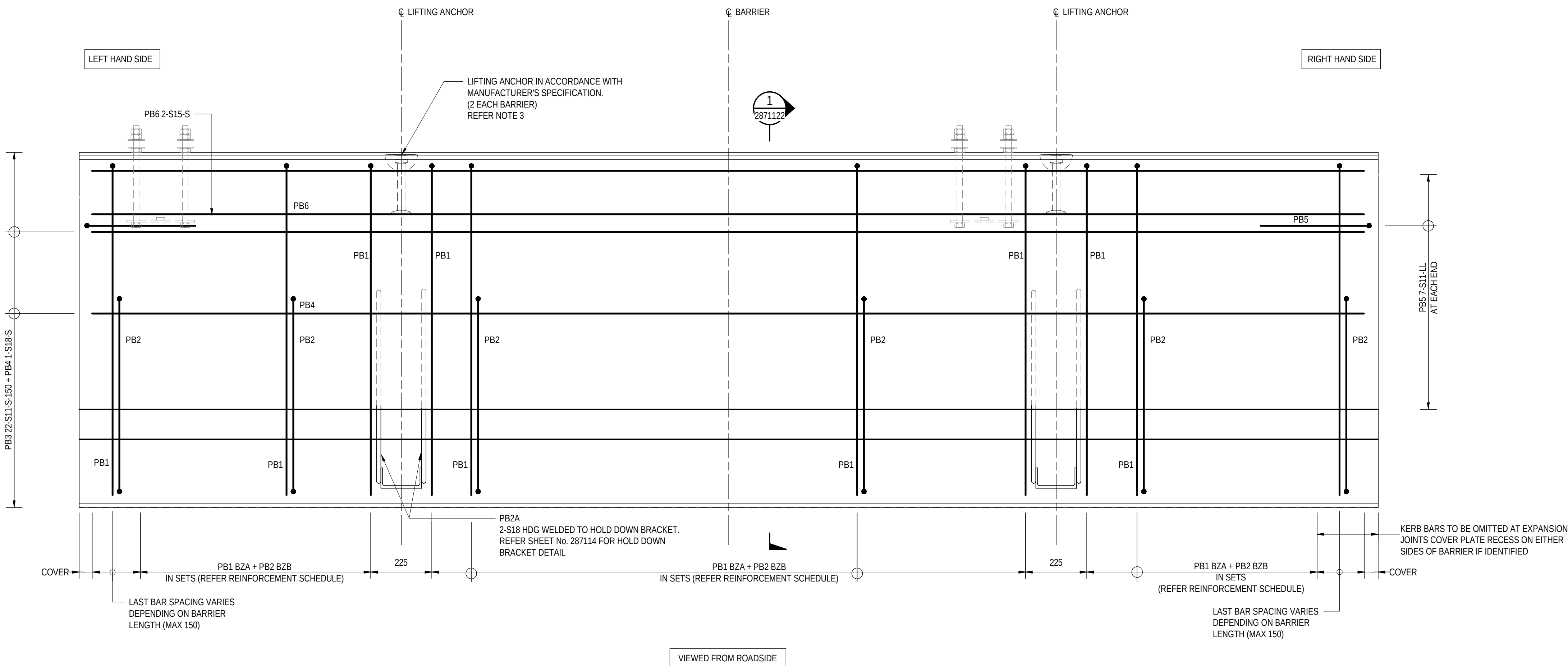
ELEVATION - PRECAST MEDIUM PERFORMANCE LEVEL BARRIER TYPE - MPB-02-B SCALE 1:10
