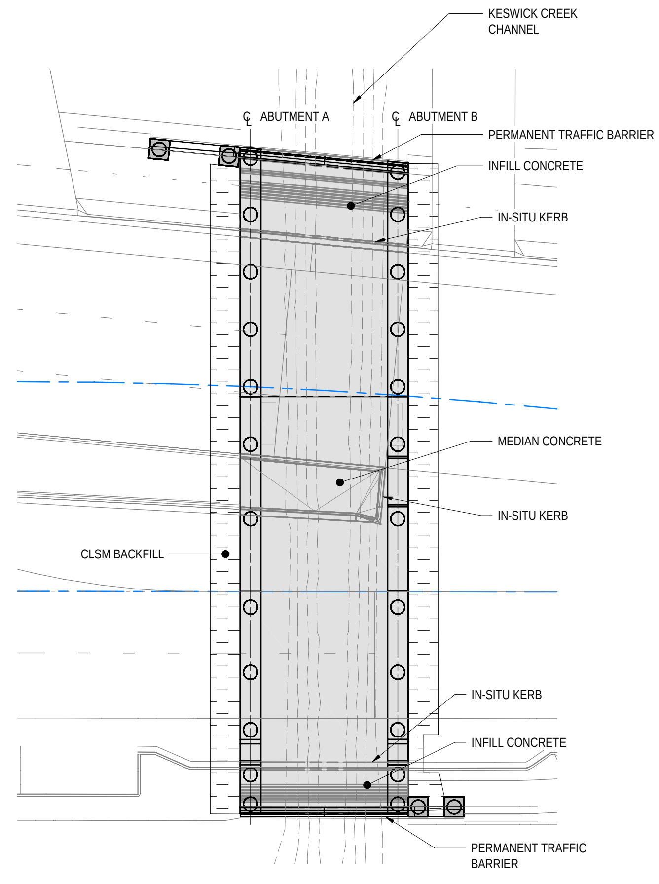
CONSTRUCTION STAGE B6
