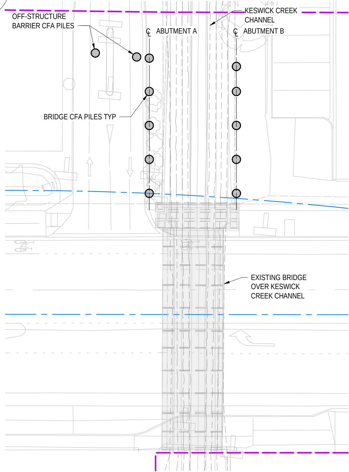
CONSTRUCTION STAGE A1
