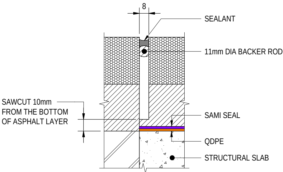
TYPICAL SEALED SAWCUT DETAIL
