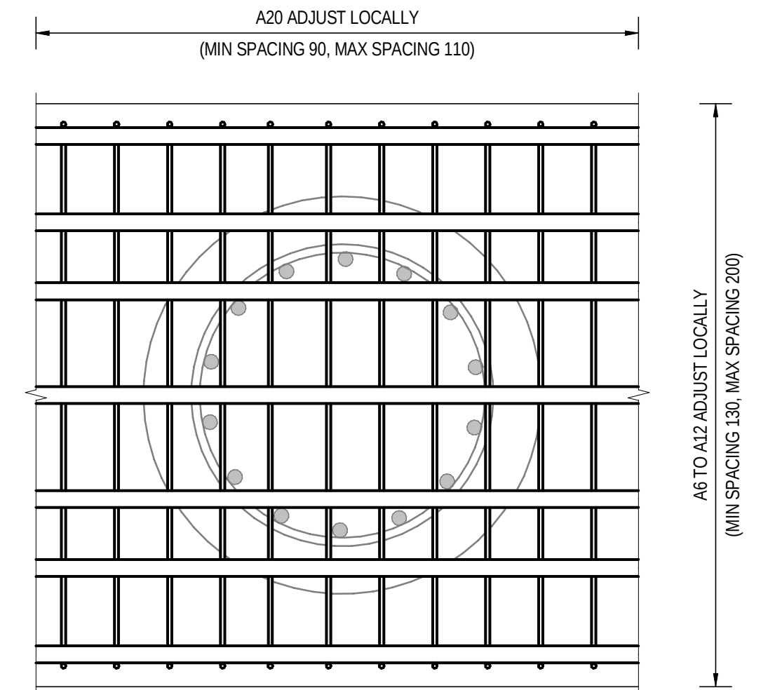
TYPICAL PLAN ABUTMENT A HEADSTOCK BOTTOM LEVEL
