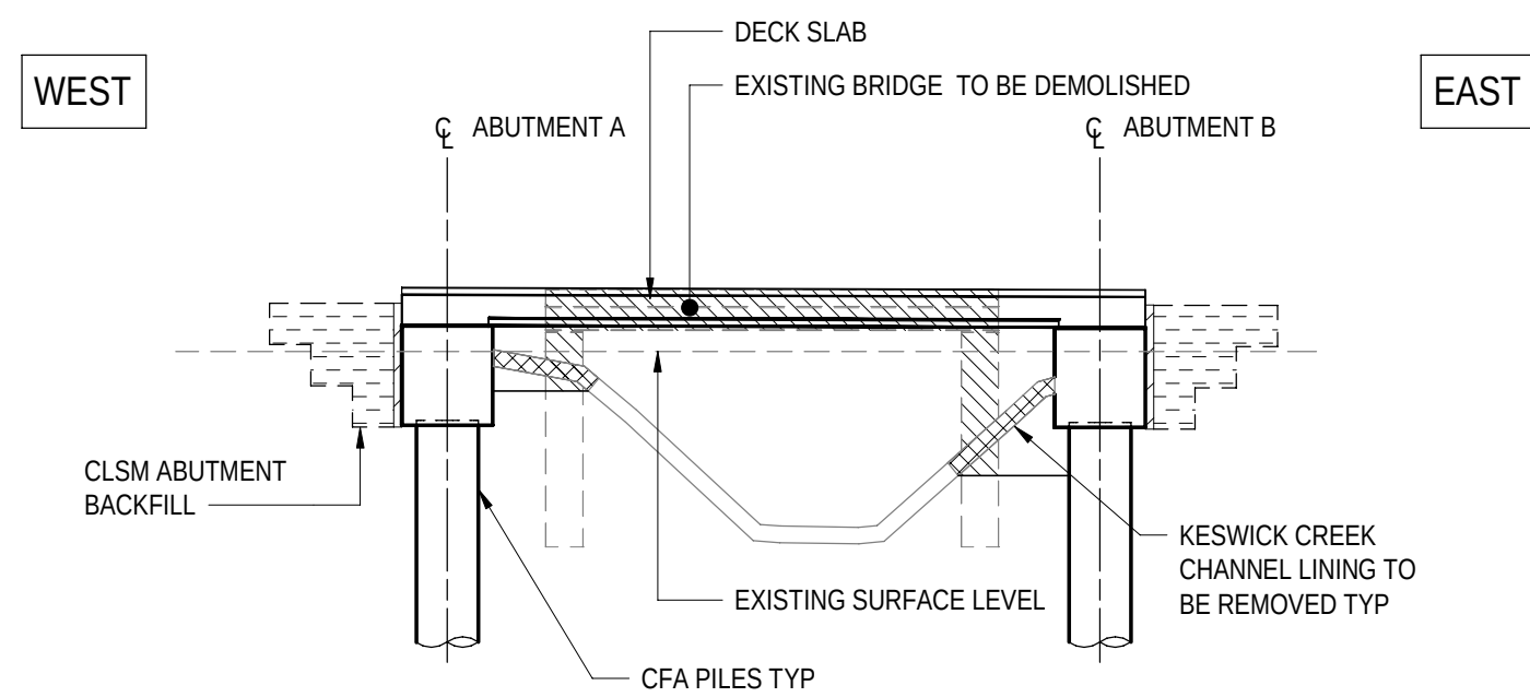
SECTION-STAGE B1
