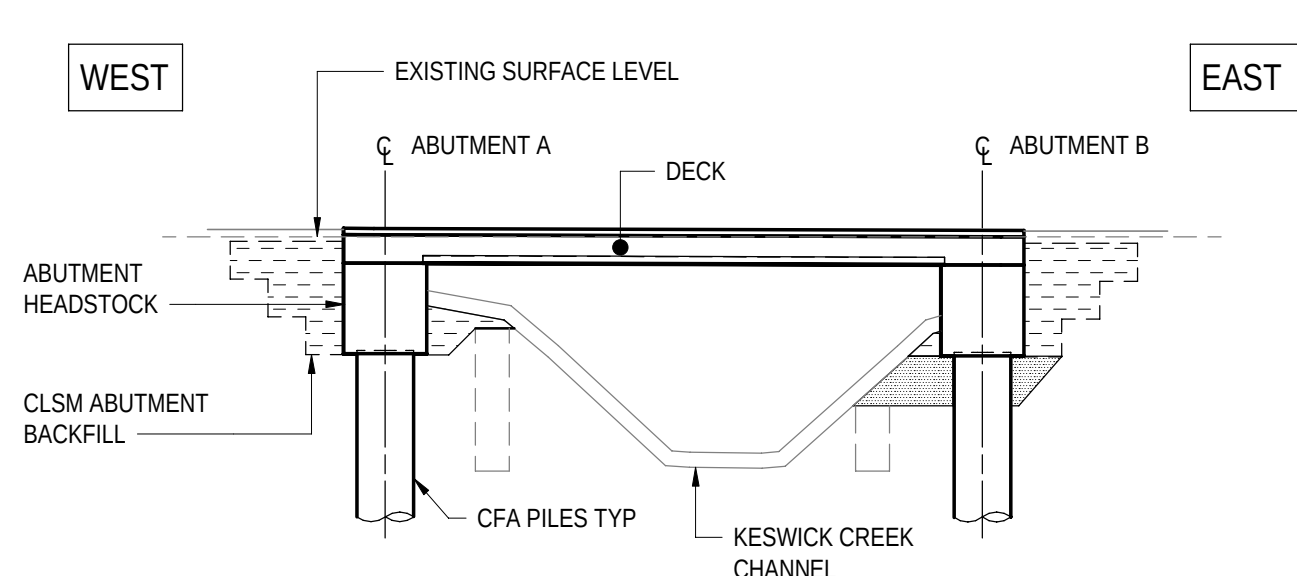
SECTION-STAGE B6
