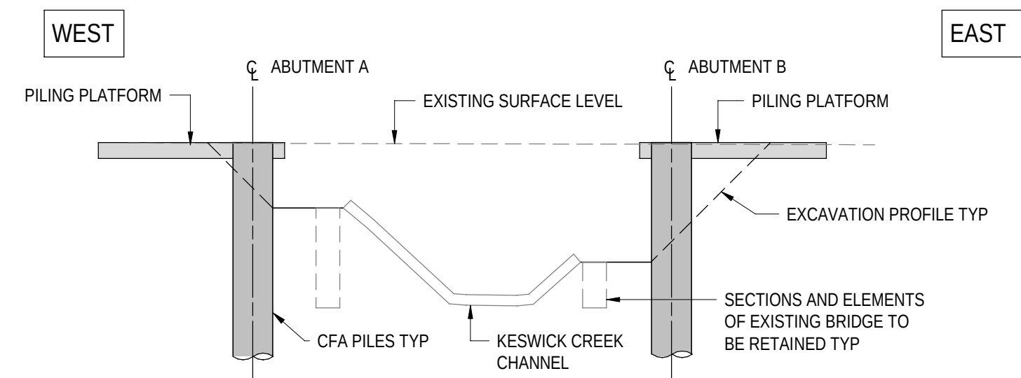
SECTION-STAGE B2
