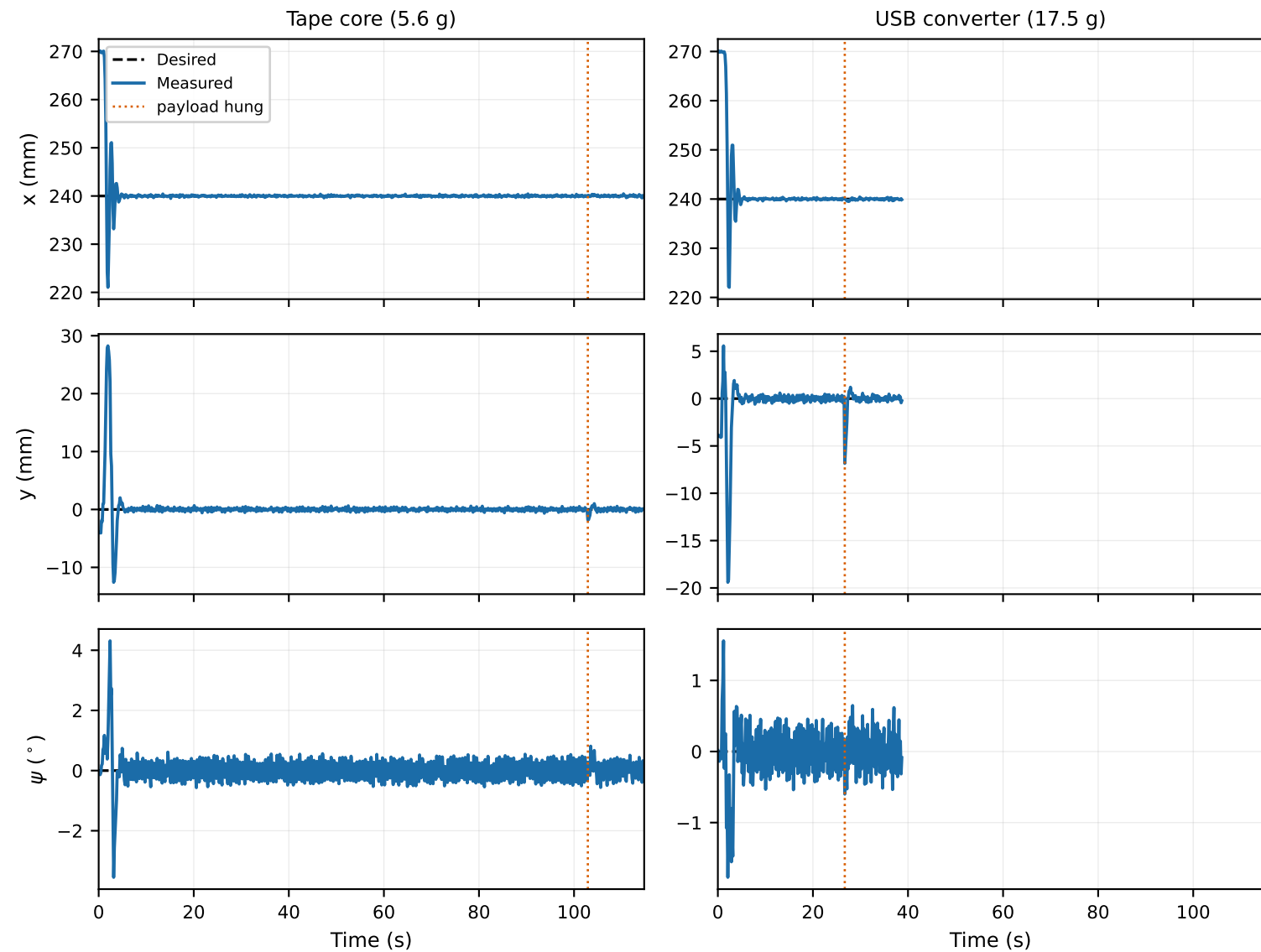
Fig. 12 - Payload disturbance while holding a stationary pose
