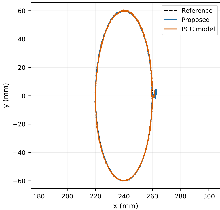
Fig. 6 - Traj. 1 - position tracking, attitude held level
