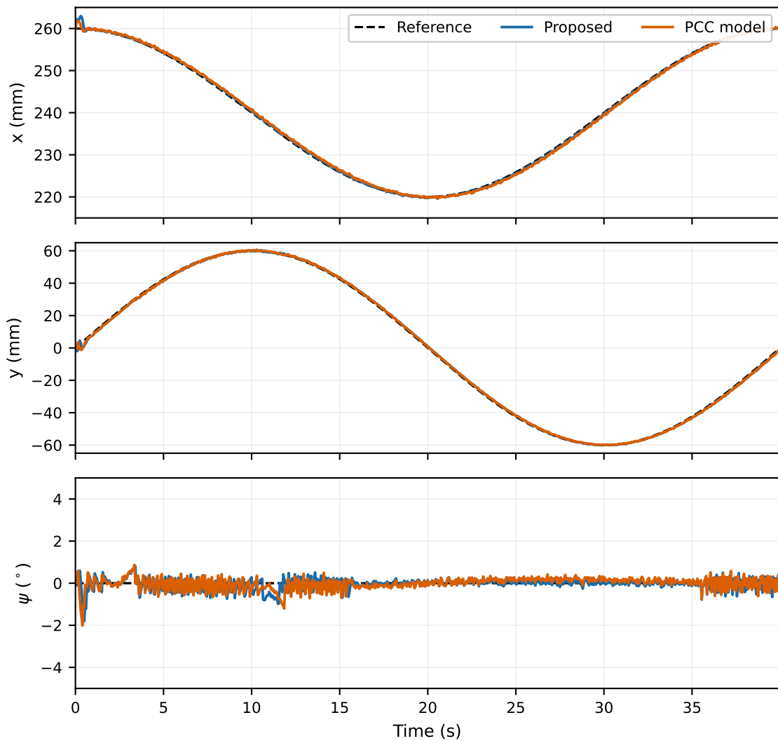
Fig. 6 - Traj. 1 - position tracking, attitude held level
