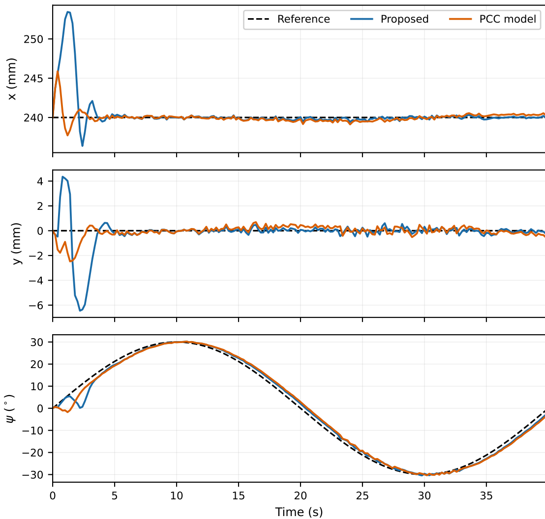
Fig. 7 - Traj. 2 - attitude tracking, position held stationary
