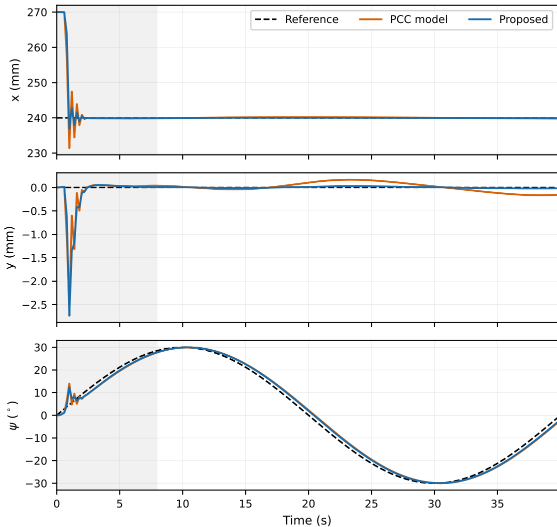
Fig. 7 - Traj. 2 - attitude tracking, position held stationary - MuJoCo plant
