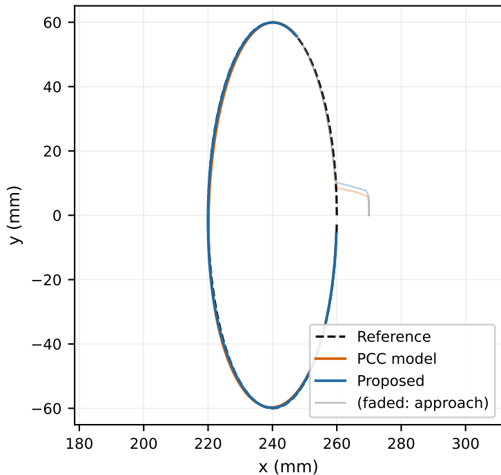
Fig. 6 - Traj. 1 - position tracking, attitude held level - MuJoCo plant
