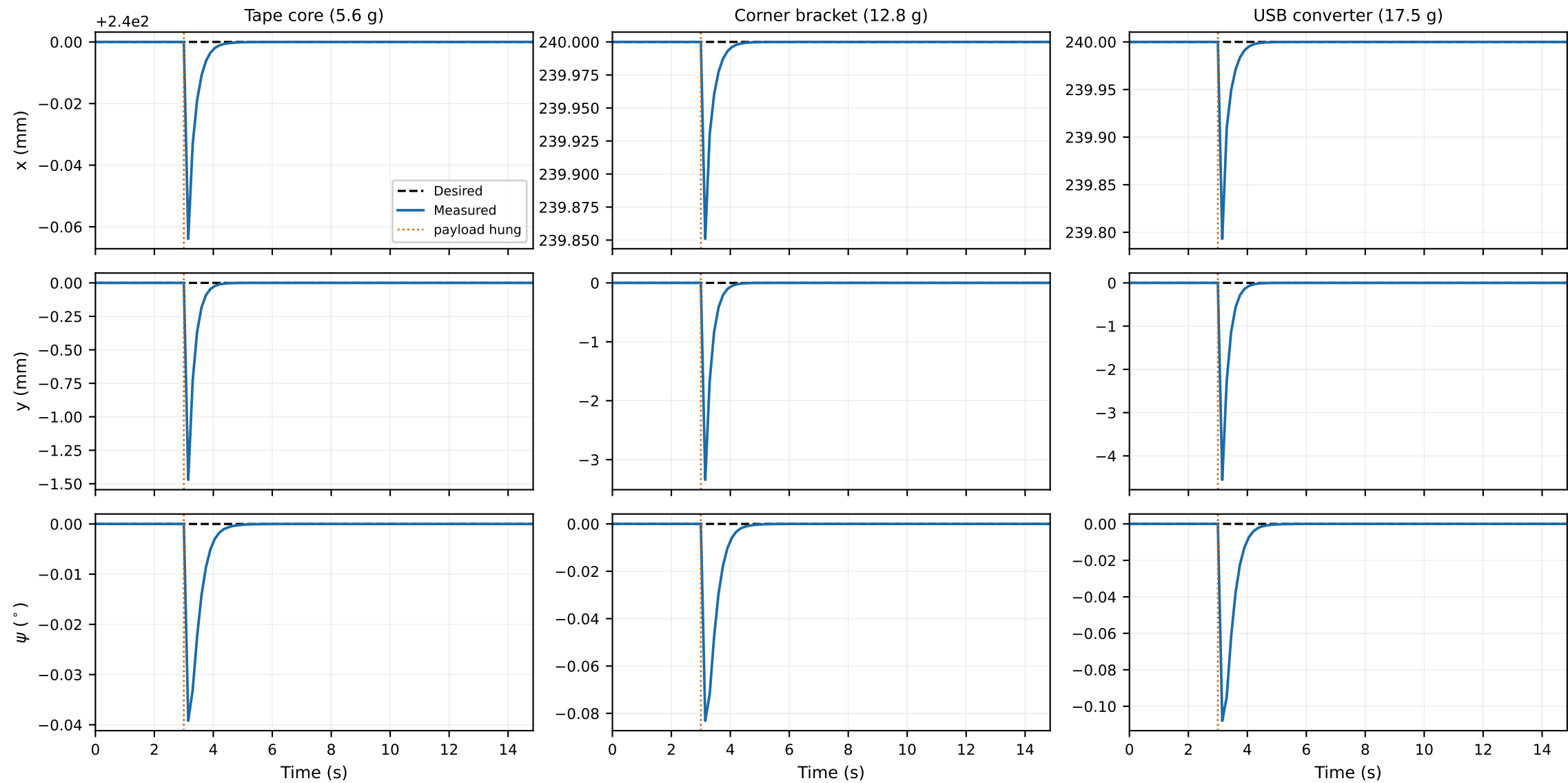
Fig. 12 - Payload disturbance while holding a stationary pose - MuJoCo plant
