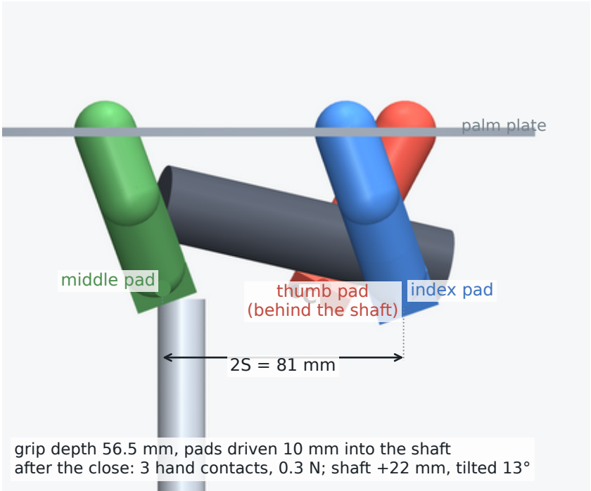
(a) grasp: the fitted grip, closed and settled
