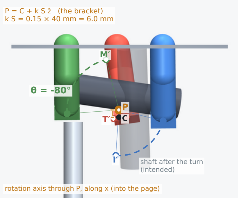
D8 sv1_w0099 k = 0.15, \theta = -80^\circ, b = 1.00 \text{ rad}
