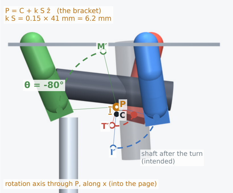
D3 sv1_u1364 k = 0.15, \theta = -80^\circ, b = 0.80 \text{ rad}
