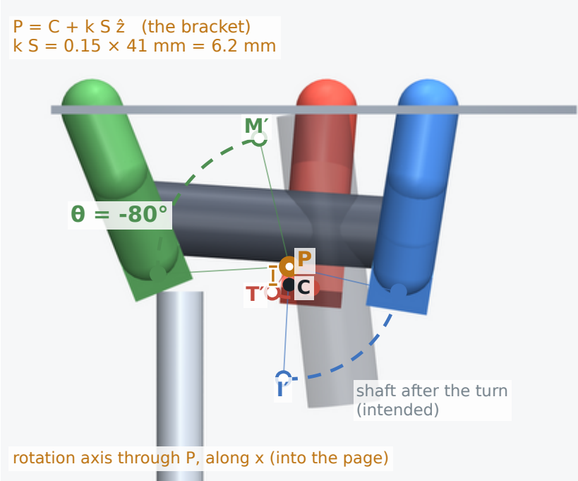
D6 sv1_u0308 k = 0.15, \theta = -80^\circ, b = 0.50 \text{ rad}
