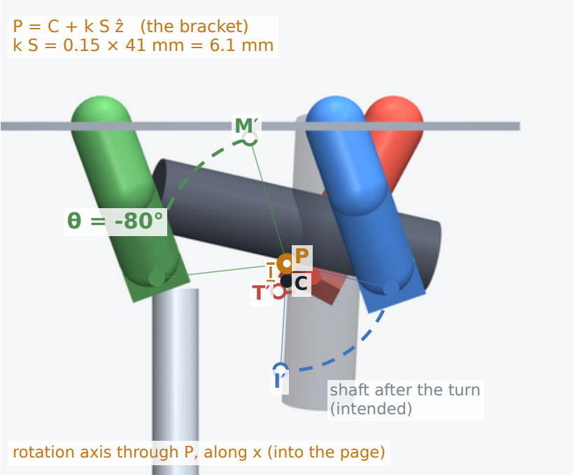
D2 sv1_w2360 k = 0.15, \theta = -80^\circ, b = 0.75 \text{ rad}
