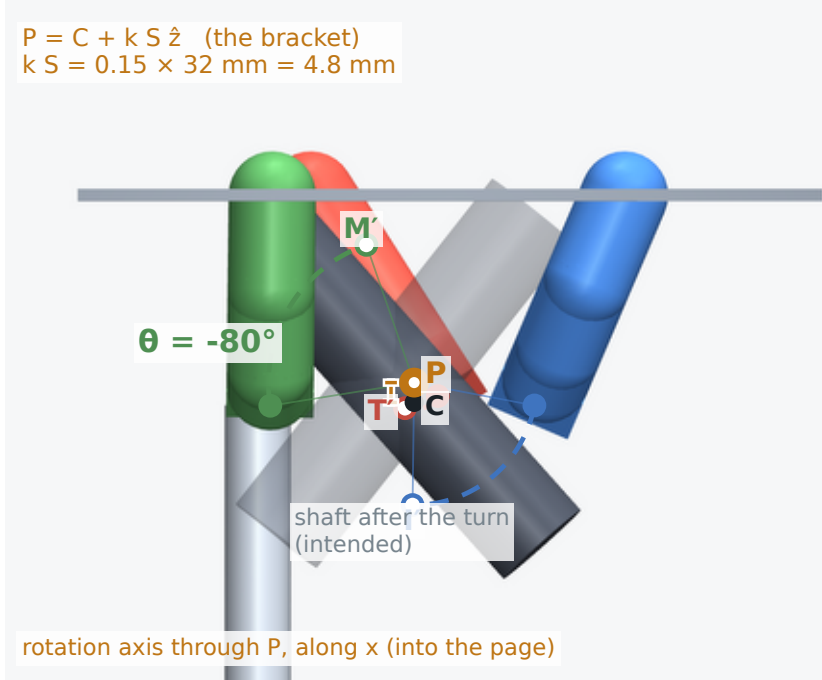
D1 sv1_w6689 k = 0.15, \theta = -80^\circ, b = 0.60 \text{ rad}
