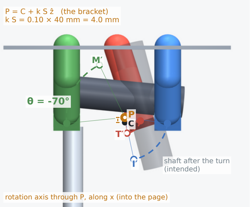
D4 g12 k = 0.10, \theta = -70^\circ, b = 0.95 \text{ rad}
