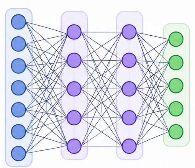
Policy Network
