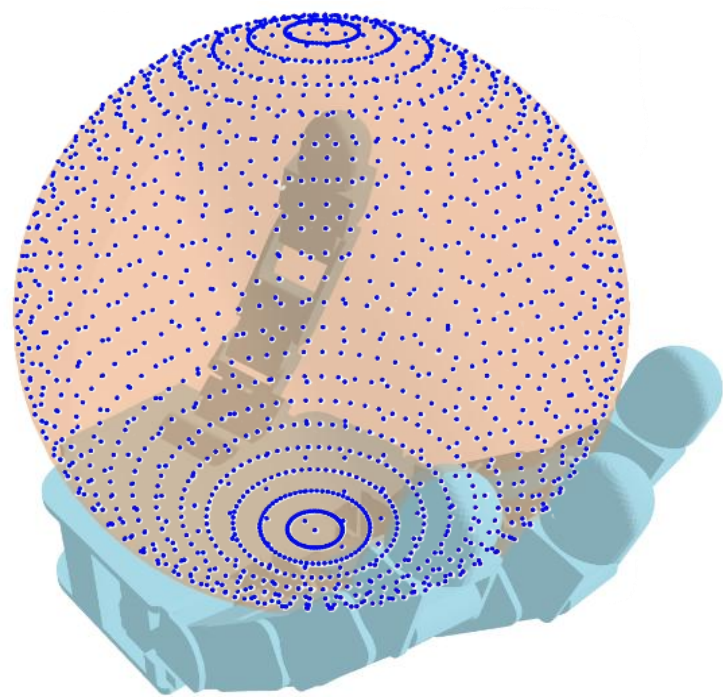
(a) Sample points on the sphere surface
