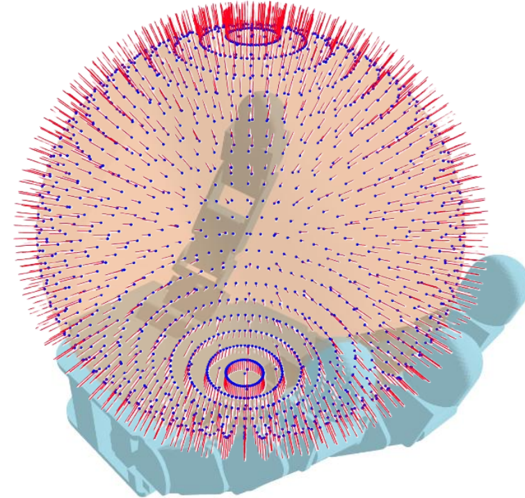
(b) Compute spherical coordinates and normals of the sampled points
