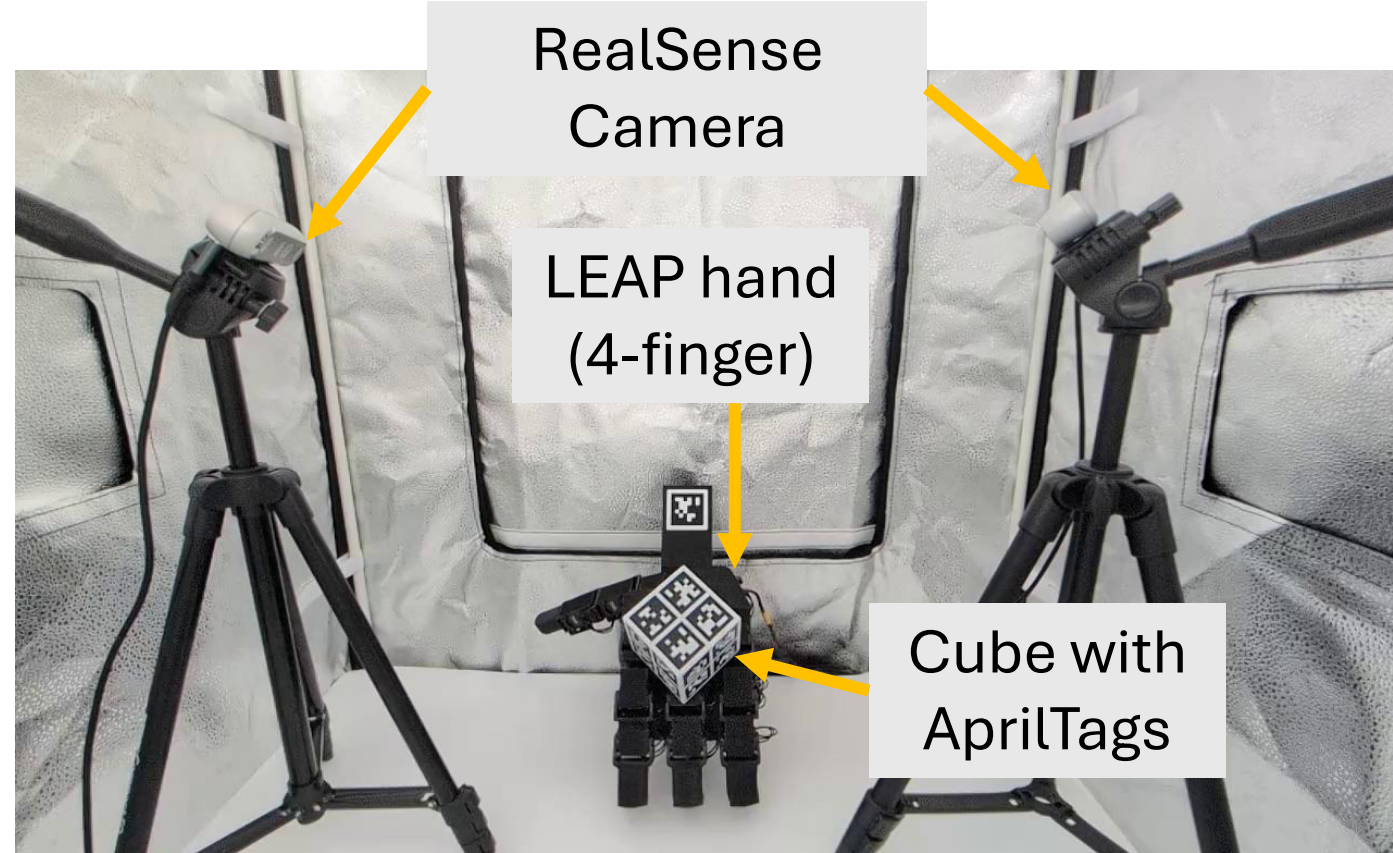
(b) Real-world Setup
