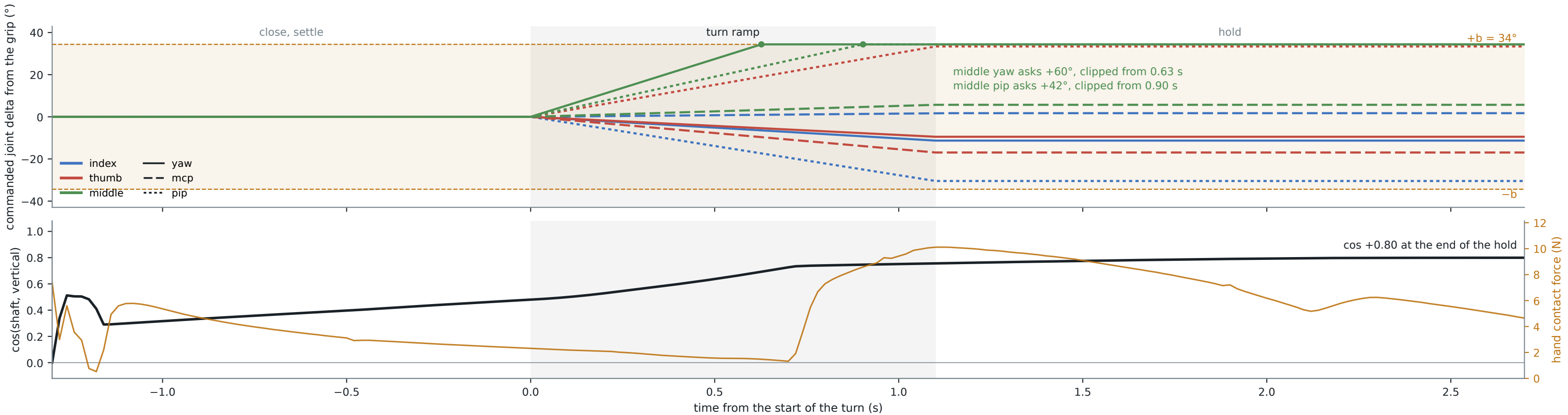
Open-loop geometric carry on D1, the construction of sv1_w6689_b060 run on the bench-calibrated plant (kp 0.5, kv 0.02): what the servos are sent and what the shaft does
