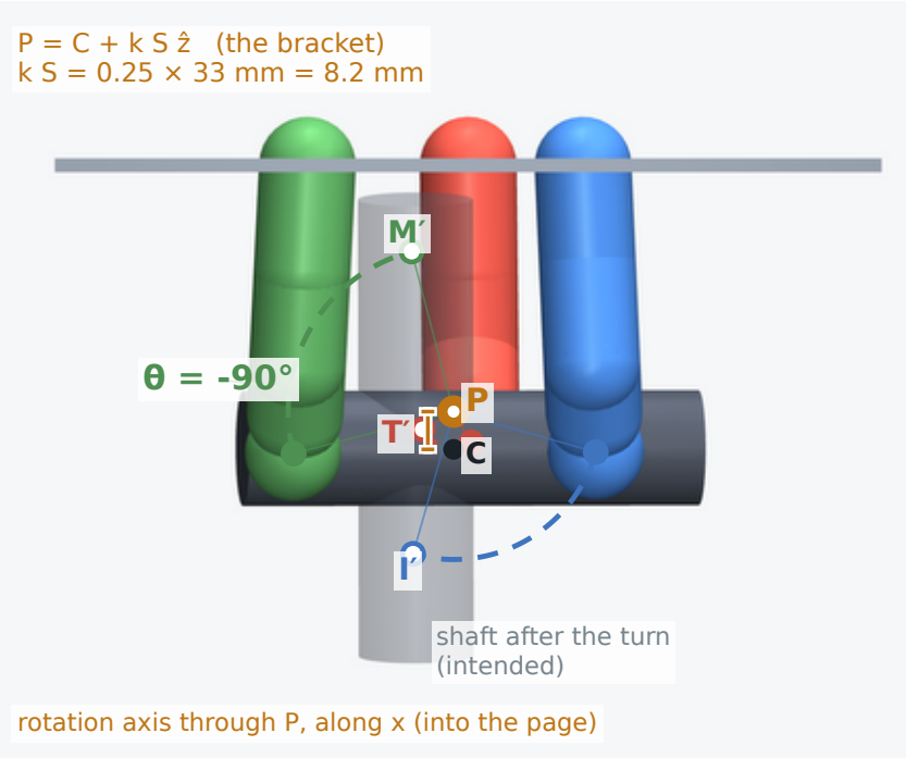
(b) construction: rotate the three pads by \theta about P
