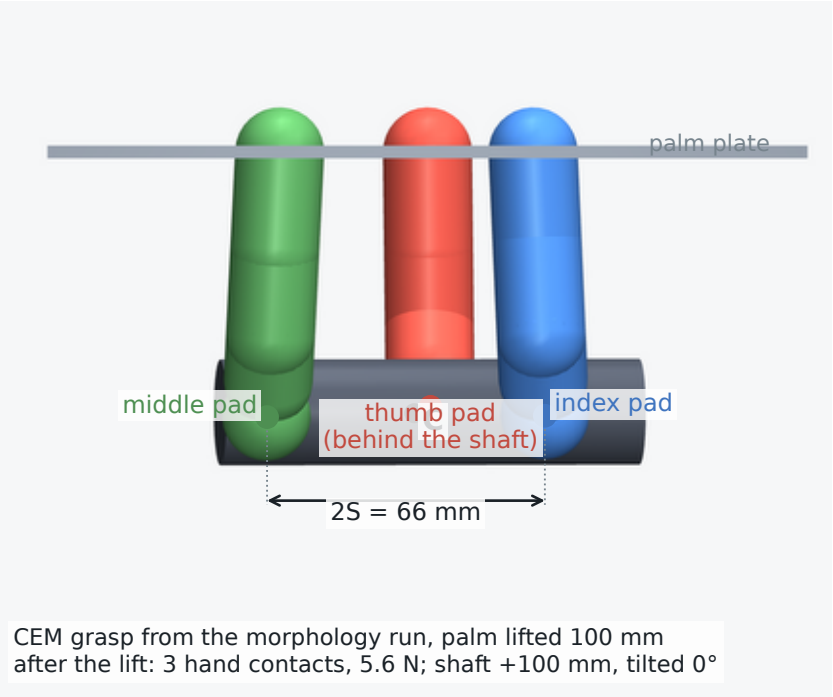
(a) grasp: the CEM grip, closed, lifted and settled
