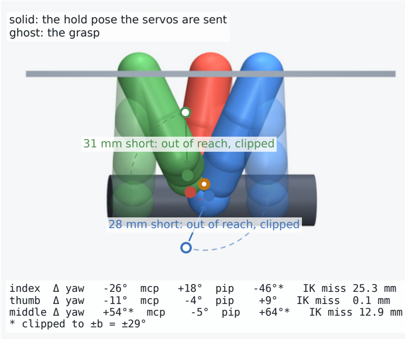
(c) hold pose: per-finger IK to l' T' M' , clipped to \pm b
