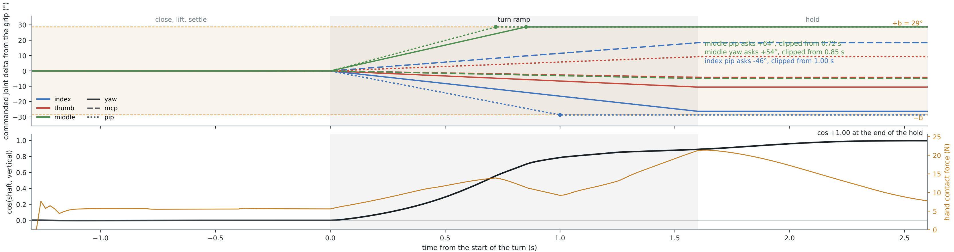
Open-loop geometric carry on D7 (rv05_manual_stored), CEM grasp, floor-free: what the servos are sent and what the shaft does
