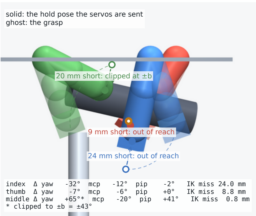
(c) hold pose: per-finger IK to I' T' M' , clipped to \pm b
