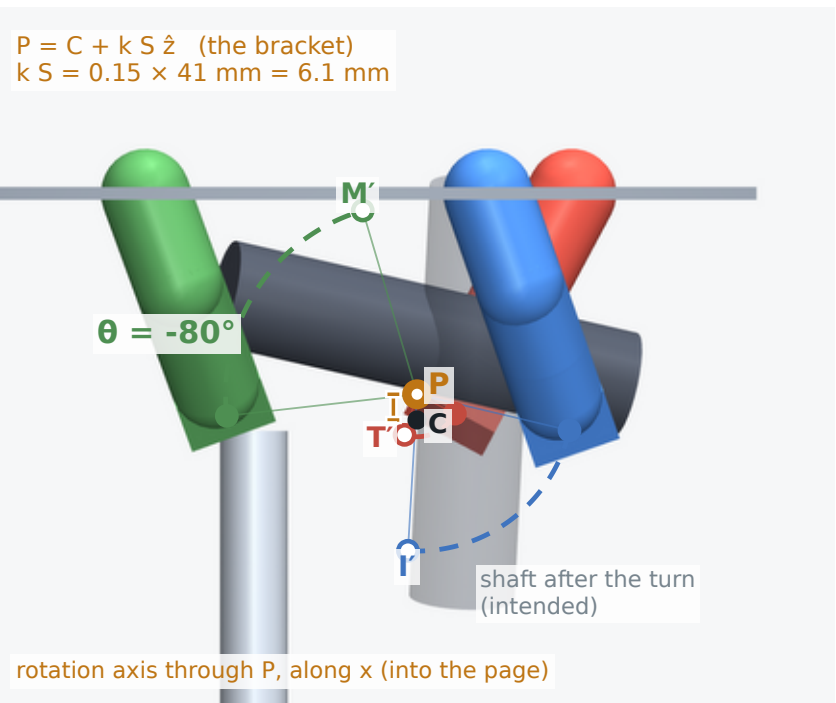
(b) construction: rotate the three pads by \theta about P
