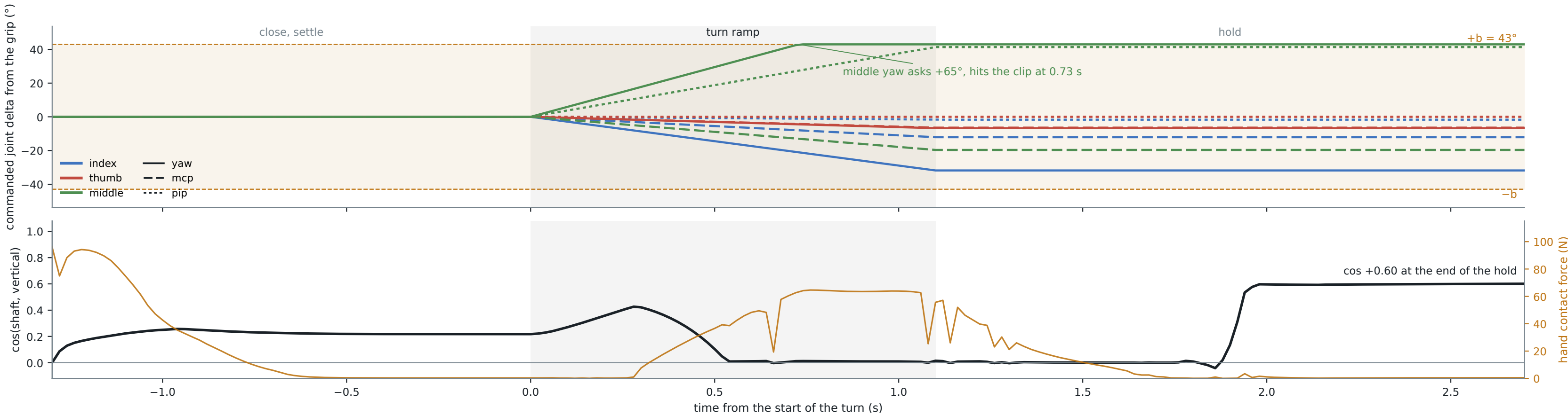
Open-loop geometric carry on D2 (sv1_w2360_b075): what the servos are sent and what the shaft does
