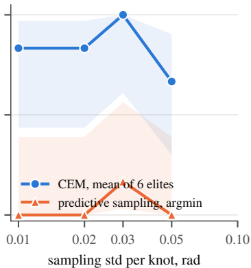
33 plans/s (6 seeds)
