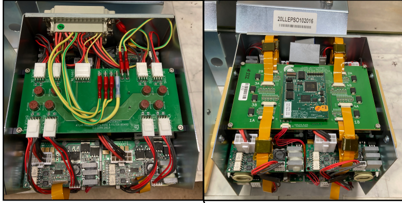
Top and bottom view of LVPS box (no lid)
